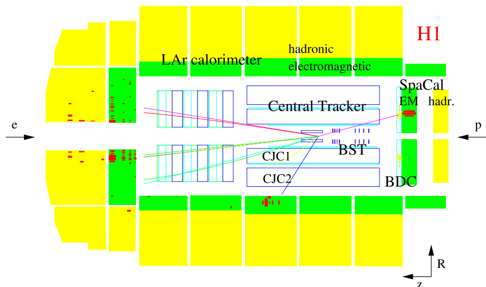
Fig. 2 A low Q^2 event as reconstructed in the H1 detector. The electron is scattered into the backward region. The electron trajectory is reconstructed in the Backward Silicon Tracker (BST) and in the Backward Drift Chamber (BDC). The electron energy is determined using the SpaCal calorimeter. The hadronic final state is detected in the central and forward tracking detectors, and in the LAr calorimeter
