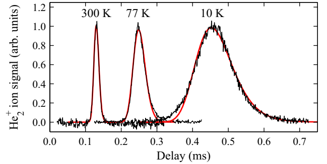
FIG. 3. (Color online) \text{He}_2^* neutral-TOF spectra obtained for temperatures of the nozzle assembly of 300 K, 77 K, and 10 K. The red curves correspond to fits to the experimental data that led to the parameters summarized in Table I. See text for details.
