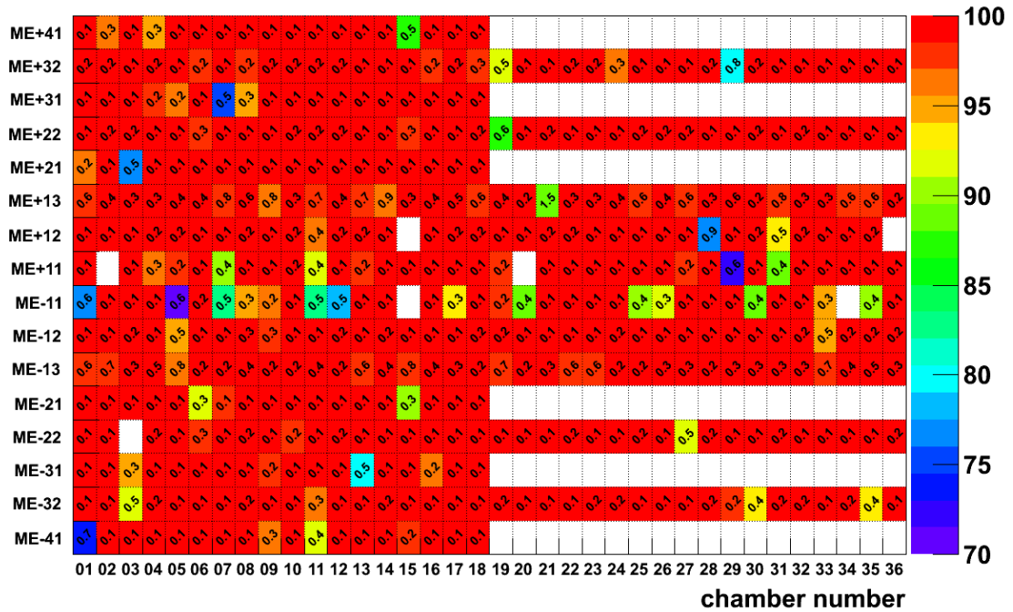
CSC Rechst efficiency (in %) CMS 2010 \sqrt{s} = 7 TeV
