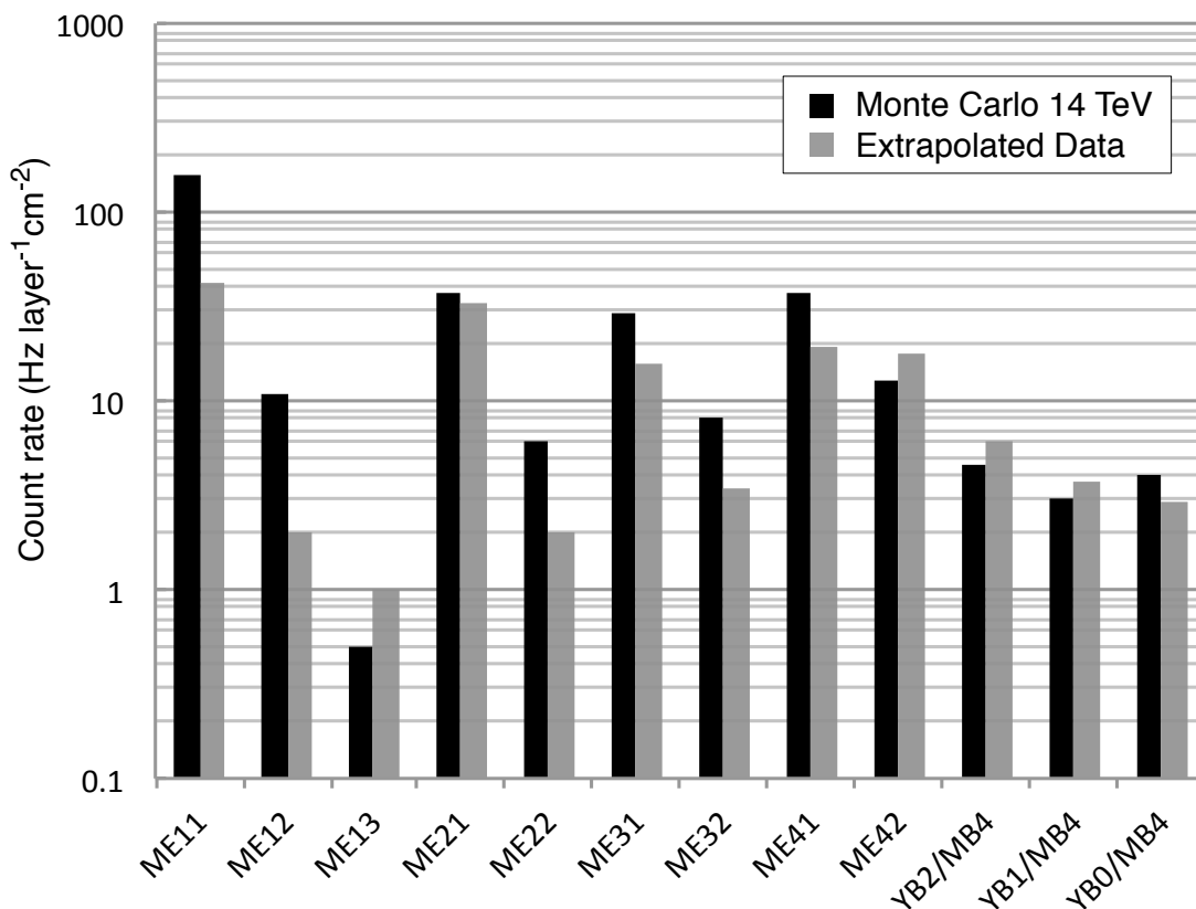
Figure 41. Radiation background rates in the CMS muon system projected for an LHC luminosity of 10^{34} \text{ cm}^{-2} \text{ s}^{-1} . The data results are linearly extrapolated from 2010 measurements at LHC luminosities up to 1.8 \times 10^{32} \text{ cm}^{-2} \text{ s}^{-1} .
