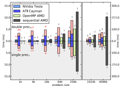
(c) 2D M'_4 interpolation
