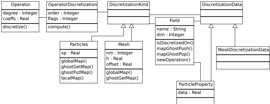
Figure 3.1. The object-oriented design of PPM core. The main abstract data types and their concrete subtypes are shown. We show a subset of the data and methods of implemented in these types.
