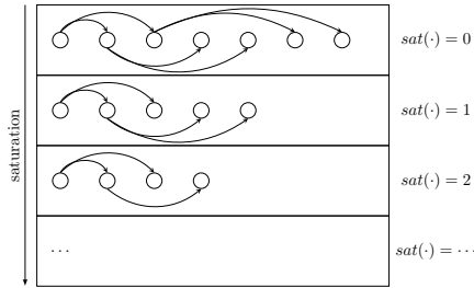
Figure 5.1. A list of heaps for fast access to vertices with maximum degree and given saturation degree.
