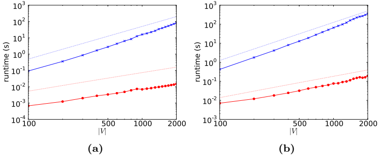
Figure 5.3. Runtime of Vizing's edge coloring (blue crosses) and heapified DSATUR (red circles) for random graphs of increasing numbers of vertices, each of which having a degree of 10 (a) or 25 (b). Heapified DSATUR performs better in both cases and scales better than Vizing's algorithm. The asymptotic runtimes of Vizing's algorithm ( O(nm) : blue) and heapified DSATUR ( O((n+m)\log m) : red) are shown as dotted lines. Heapified DSATUR is applied to G = L(\tilde{G}) while Vizing is directly applied to \tilde{G} .
