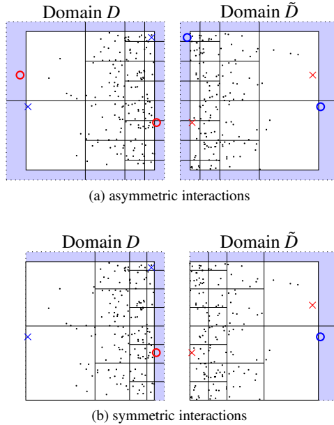
Figure 4.4. Halo layers for symmetric and asymmetric neighbor lists and treatment of periodic boundary conditions. The computational domain is decomposed into two (sub-)domains D and \tilde{D} (cf. Fig. 4.1). On each (sub-)domain and its respective halo layers, a separate AR cell tree (black lines) is built. Blue crosses indicate particles in domain D that are ghosts in the halo layer of domain \tilde{D} (blue circles). The red crosses highlight two particles from domain \tilde{D} that are ghosts on domain D (red circles). For each color, two example-particles are shown: one for periodic boundary conditions, the other for internal (sub-)domain boundaries.
