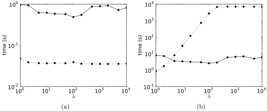
Figure 4.7. Total runtime for increasing resolution spans 1 \leq \lambda \leq 10\,000 and constant N = 10^6 . (a) Runtime for constructing conventional (dashed line) and AR (solid line) cell lists in 2D. (b) Total runtime for constructing conventional (dashed line) and AR (solid line) cell list and constructing Verlet list based on them.
