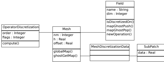
Figure 3.3. The mesh data type and associated types. We show a subset of the data and methods of implemented in these types.
