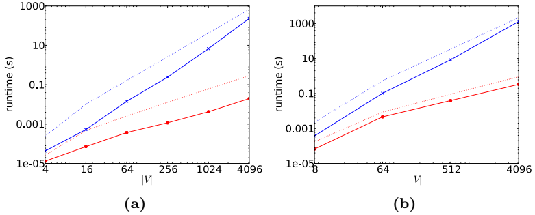
Figure 5.5. dsatur (red) and vizing (blue) runtime performance benchmarks on a cartesian mesh in 2D with 8-neighborhood (a) and 3D with 26-neighborhood (b). Asymptotic runtimes for Vizing's algorithm ( O(nm) : blue) and heapified DSATUR (on line-graphs, O((n+m) \log m) red) are shown in dotted lines.
