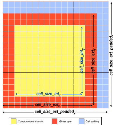
Figure 6.9. Sizes of the computational domain ( cell\_size\_int ), including ghost layers ( cell\_size\_ext ), and after padding with extra cells ( cell\_size\_ext\_padded ) for consecutive memory access. Extended blocks are shown by black lines.
