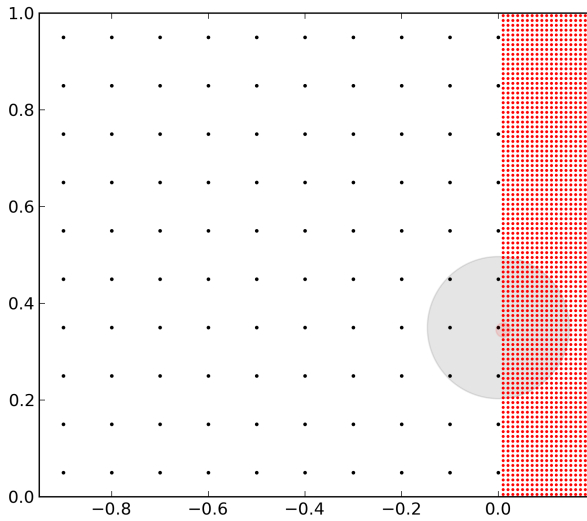
Figure 4.5. An example particle distribution used for the present benchmarks. In this figure N = 2000 and \lambda = 10 . The “large” black particles have a cutoff radius of 0.15, while the “small” red particles have a cutoff radius of 0.015 ( \lambda = 0.15/0.015 = 10 ). For comparison, the interaction ranges of two neighboring particles at the resolution interface are shown as shaded circles of the respective color.
