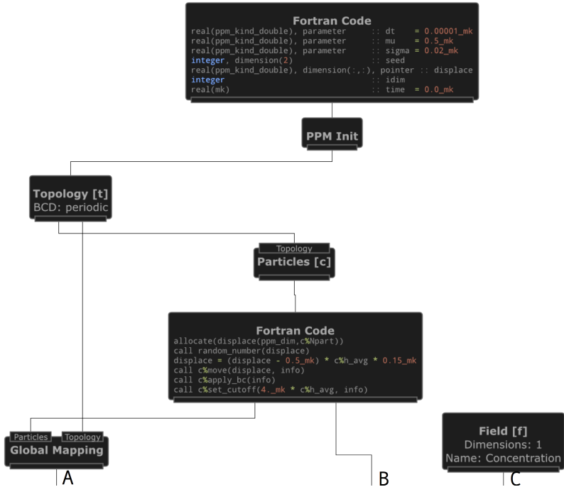
Figure C.1. The initialization part of the program. A topology and a particle set is created. The particles are mapped onto the topology and the the field f is created. The diagram also shows Fortran code blocks providing code that is not expressed in PPML.
