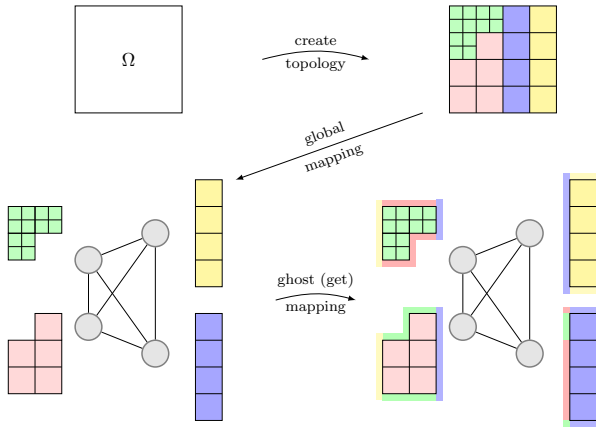
Figure 2.1. In PPM the computational domain \Omega (upper-left ) is decomposed and subdomains are assigned to processors (upper-right ). Particles and meshes are then mapped onto this topology using a global mapping (lower-left ). Ghost layers are communicated by ghost mapping (lower-right ). In this example periodic boundary conditions are assumed.
