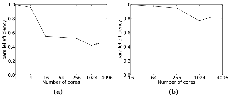
Figure 8.2. Parallel efficiency of a weak scaling of the PPML reaction-diffusion client. The largest cores of processors used was 1936. All cores per node are used. This leads to a performance drop at 16 cores (a). (b) The parallel efficiency when starting from 16 processes.
