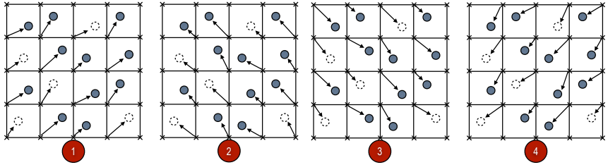
Figure 6.11. Mesh-to-particle interpolation example in 2D with a linear interpolation function (support size 4). In each of the 4 iterations, the work items in the same workgroup (block) accumulate on their particles the contributions from the mesh nodes in the same direction. Dummy particles (dashed circles) avoid conditional statements. The 4 stages are repeated p_{\max} times until all particles have been considered.
