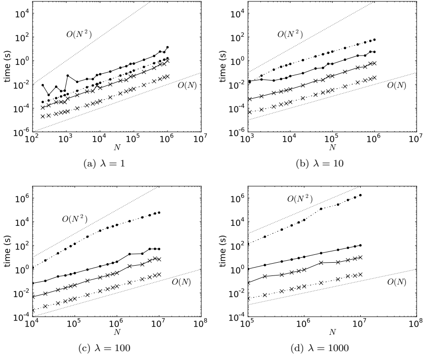
Figure 4.6. Runtime for increasing numbers of particles N and resolution spans \lambda = [1, 10, 100, 1000] (a–d). Each plot shows the total runtime for constructing (crosses) conventional (dashed lines) and AR (solid lines) cell lists in 2D and for constructing the cell lists plus constructing Verlet lists based on them (dots). The theoretical slopes of an O(N) and an O(N^2) algorithm are indicated by the dotted lines.
