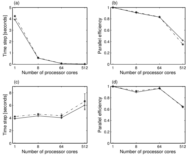
Figure 3.4. Benchmark of a PPM client simulating diffusion in complex shapes. Average (symbols) and standard deviation (error bars) of the maximum (over all processor cores) wall-clock time per time step, sampled over 100 steps, and parallel efficiency for the old (dashed lines) and new (solid lines) PPM core implementation. (a) and (b) show the results for a fixed-size problem with 2.1 million particles (strong scaling); (c) and (d) for a scaled-size problem starting with 2.1 million particles on 1 processor and going to 1.1 billion particles on 512 processors (weak scaling). All tests were done in a cubic domain using equi-sized and perfectly load-balanced subdomains in order to test the performance of the PPM implementation rather than that of the implemented decomposition algorithms.
