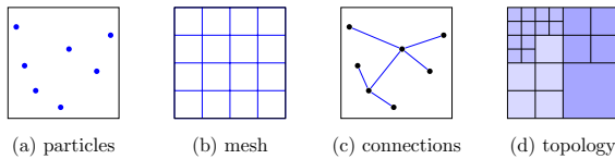
Figure 7.1. PPM provides four types of data abstractions: particles (a), meshes (b), connections (c), and topologies (d). Hybrid particle-mesh simulations can be expressed in terms of particles and meshes. Connections allow particle-particle associations, representing for example covalent bonds in molecular dynamics, contact lists in discrete element methods, or graph edges in social networks.
