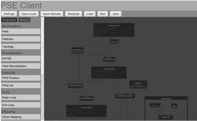
Figure 7.4. The main webCG interface. On the left, the block list and property editor view are seen. On the top, the main menu bar and the project title are placed. The interface is dominated by the SVG block-diagram editor.
