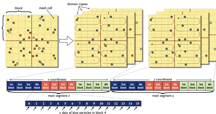
Figure 6.6. Particle data are stored in buffer segments, blocks, and domain copies according to their dimension, mesh cell index, and number of fellow particles within the mesh cell. Particles within the same mesh cell are stored in different domain copies as highlighted by color. Each domain copy is subdivided into blocks (red dashed lines) that are stored consecutively in the buffer. Within each block, particles are numbered in the order shown by the dashed arrows. Data along different space dimensions are stored in separate main segments of the buffer.
