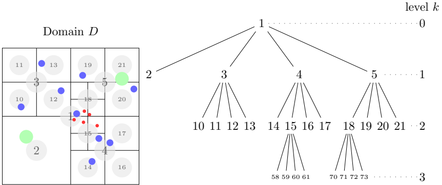
Figure 4.2. Left: sketch of an AR cell list with large (green), medium (blue), and small (red) particles. The domain D is adaptively subdivided (black lines). Right: The corresponding cell tree with cells c_k on levels k and level-order indices J(c_k) , corresponding to the numbers given in the gray circles in the left panel.
