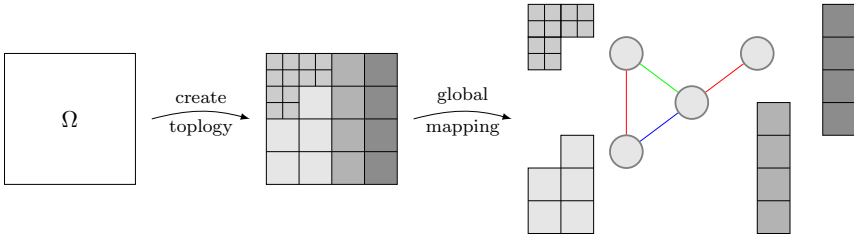
Figure 5.2. First, we create a topology for the computational domain \Omega (left panel) by decomposing it into subdomains and assigning them to processors (center panel). Then, we map the data onto this topology. The subdomain neighborhood defines a processor neighborhood (right panel). This neighborhood is abstracted as a graph \tilde{G} = (V, E) , where V is the set of processors and E = \{(v_i, v_j) \mid v_i, v_j \text{ have neighboring subdomains}\} . An edge-coloring of \tilde{G} is computed by applying the vertex coloring algorithm DSATUR (Algorithm 5.1) to the line-graph G = L(\tilde{G}) . Free space boundary conditions are assumed.
