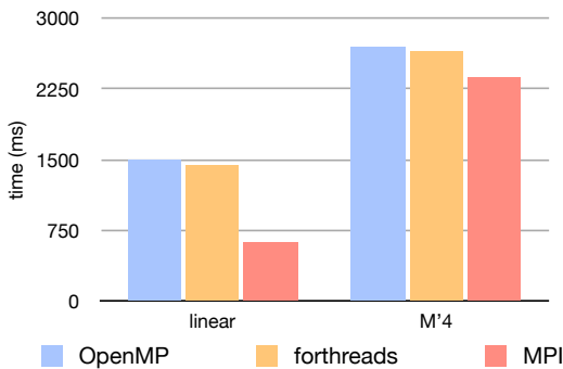
Figure 6.3. Timings for particle-mesh linear and M^4 interpolation using OpenMP (blue), forthreads (orange) and MPI (red). All timings were performed on an AMD Opteron 8380 using 8 threads on 8 cores. The used problem size is 512 \times 512 \times 512 with 1 particle per mesh cell.
