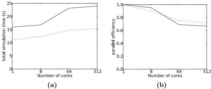
Figure 3.5. Wall-clock time (a) and parallel efficiency (b) of a molecular dynamics simulation benchmark client using the latest object-oriented PPM core library (solid line) and the backported code using the original PPM library (dashed line) on a scaled-size problem with 1 million particles per core (weak scaling). All tests were done in a cubic domain using equi-sized and perfectly load-balanced subdomains in order to test the performance of the PPM implementation rather than that of the implemented decomposition algorithms.
