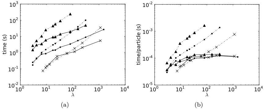
Figure 4.9. Runtime for constructing the cell lists and using them to construct Verlet lists for the test case shown in Fig. 4.8. For both conventional (dashed lines) and AR (solid lines) cell lists we vary the resolution span \lambda and the mean resolution h_0 on the larger sphere, hence varying the total number of particles N . Crosses, dots, and triangles correspond to h_0 = 0.1, 0.2 , and 0.45 , respectively. Note that N increases with \lambda . The two panels show: (a) the total runtime and (b) the runtime per particle.
