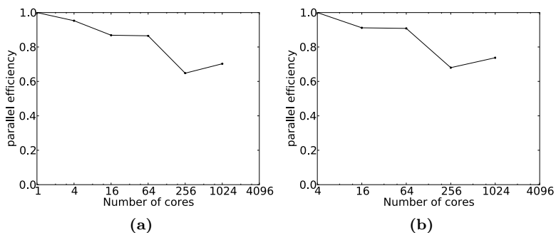
Figure 8.3. Parallel efficiency of a weak scaling of the PPML reaction-diffusion client on up to 1024 processes. In order to avoid memory congestion, we use only 1 core per processor. (a) Parallel efficiency with respect to the sequential run. (b) Parallel efficiency relative to the largest run using only one node.
