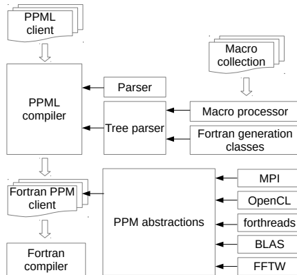
Figure 7.3. The PPML framework. Line arrows represent “used by” relationships, hollow arrows show the processing order. The PPML compiler is supported by the parser and the tree parser, which in turn uses the PPML macro collection and the Fortran generation classes to expand PPML operations to Fortran source code.
