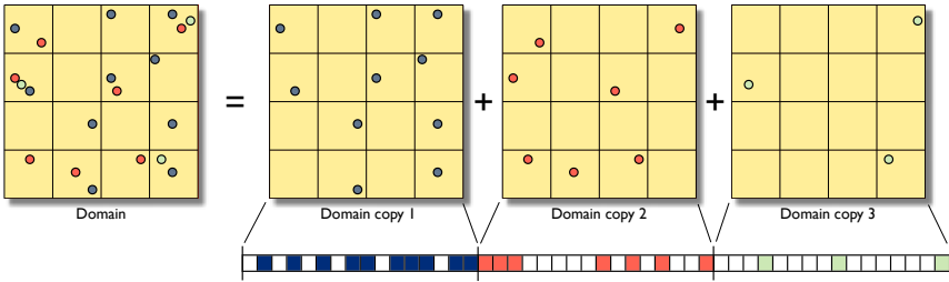
Figure 6.7. Illustration of the use of domain copies and dummy particles in order to avoid conditional statements and guarantee coalesced memory access. See main text for details.
