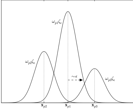
Figure 1.1. Three particles \mathbf{x}_{p1} , \mathbf{x}_{p2} , and \mathbf{x}_{p3} carrying Gaussian mollification kernels \zeta_\epsilon with strengths \omega_{p1} , \omega_{p2} , and \omega_{p3} .
