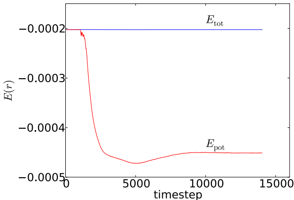
Figure 8.6. Total (blue) and potential (red) energy of 1 million particles over 14,000 time steps in a PPML Lennard-Jones simulation.
