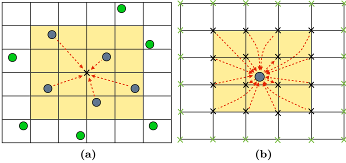
Figure 1.2. Schematic of (a) particle-to-mesh and (b) mesh-to-particle interpolation in 2D using an interpolation function with support \pm 2\mathbf{h} (support region is shaded in yellow). Blue particles ( \mathcal{P}(m) ) and mesh nodes ( \mathcal{M}(p) ) are within the support region of the center node/particle and hence assign onto it. Green particles and nodes lie outside the support and are not considered.
