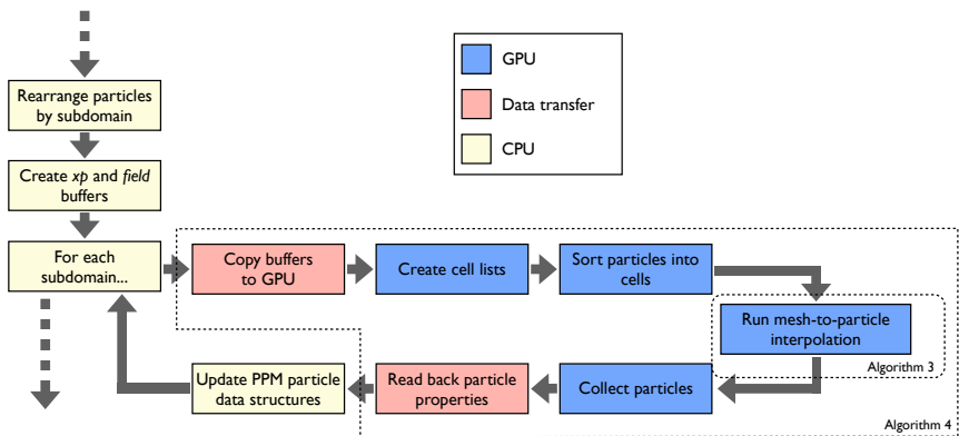
Figure 6.13. Workflow scheme for GPU-accelerated mesh-to-particle interpolation in the PPM library.
