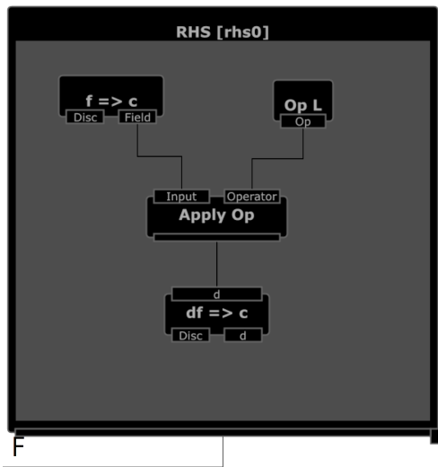
Figure C.3. Inside the right-hand side function we apply the DC-PSE discretized Laplacian operators to the particle set.
