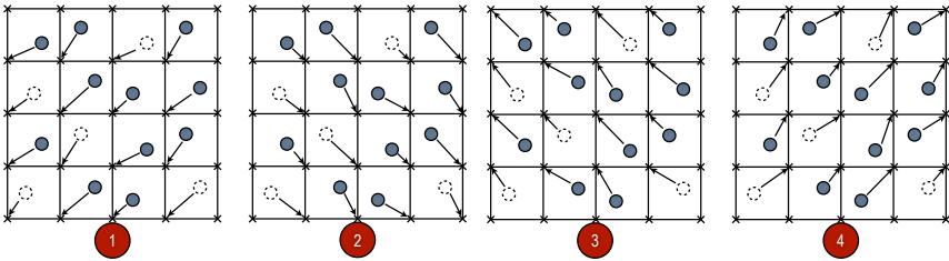
Figure 6.10. Particle-to-mesh interpolation example in 2D with a linear interpolation function (support size 4). In each of the 4 iterations, the work items in the same workgroup (block) update the mesh nodes in the same direction in order to avoid concurrent writes. Dummy particles (dashed circles) avoid conditional statements. The 4 stages are repeated p_{\max} times until all particles have been assigned.
