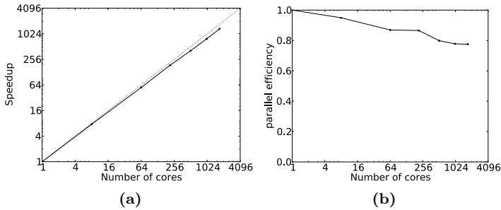
Figure 8.7. Speedup and parallel efficiency of the PPM Lennard-Jones benchmark client. The parallel efficiency remains at 77.5% on 1728 processes.
