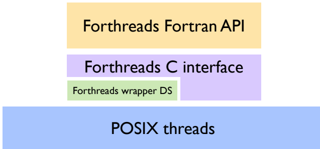
Figure 6.2. The forthreads library consists of two parts. First, the pthreads functions and opaque types are wrapped with C code that exposes Fortran-friendly data types and function interfaces. Then, a set of Fortran routines provides the user with a seamless Fortran-native interface calling internally the forthreads C functions and passing all necessary pointers and data.
