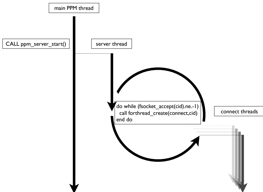
Figure 6.4. PPM server. The arrows visualize the thread control flow; dashed lines are thread spawns. The PPM server creates a thread for the server listen loop and for each newly established connection.
