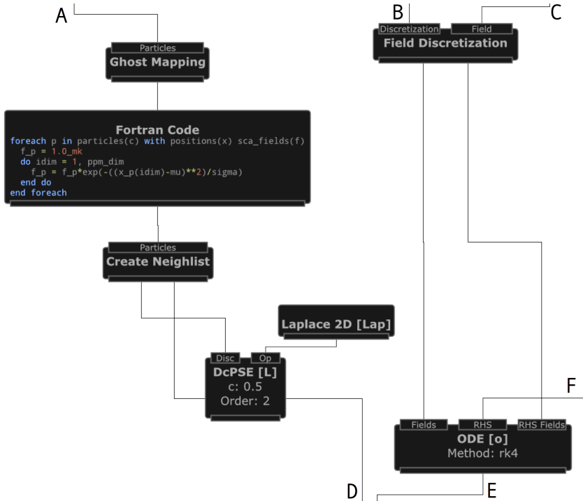
Figure C.2. The field is discretized onto the particles and a ghost-get mapping is performed. Then, we compute the Verlet list on the particle set and create the DC-PSE operators of order 2. The ODE object is created, taking the right-hand side and the field f as arguments.
