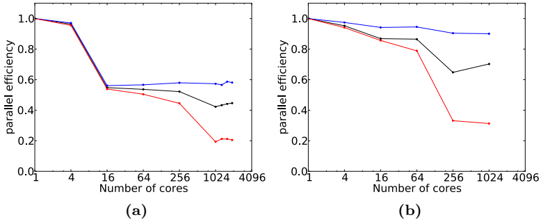
Figure 8.4. Parallel efficiency of a weak scaling of the PPML reaction-diffusion client using 16 cores per node (a) and four processors per node (b). In addition to the average efficiency, we show the efficiencies of the fastest processor in blue, and of the slowest processor in red.
