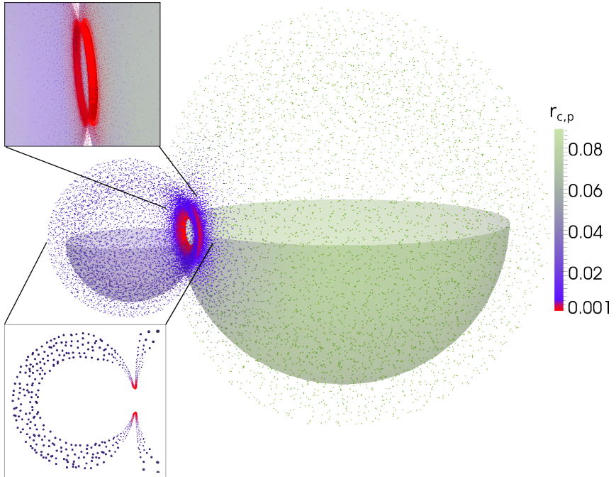
Figure 4.8. Particle distribution used in the present example of an adaptive-resolution simulation of diffusion on a surface. The surface is axially symmetric and only its lower half is shown. The surface is represented as a level set discretized on the particles and restricted to a narrow band. Both the width of the narrow band and the cutoff radii of the particles, represented by the color code, depend on the local surface curvature. The high curvature at the neck between the two sphere shells requires a locally increased resolution.
