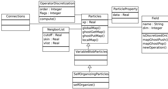
Figure 3.2. Class diagram of the PPM particles type and associated types. We show a subset of the data and methods of implemented in these types.
