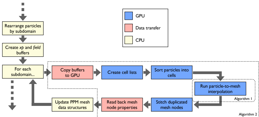
Figure 6.12. Workflow scheme for GPU-accelerated particle-to-mesh interpolation in the PPM library.
