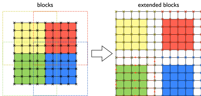
Figure 6.8. Mesh nodes close to the boundary of a block are replicated in order to avoid concurrent writes and race conditions. Left: the dashed squares indicate the areas within which mesh nodes are influenced by particles in the block of the same color. Right: extended blocks are defined by replicating mesh nodes in overlapping influence regions. The red dashed arrow shows the storage order of the mesh nodes inside the green extended block.
