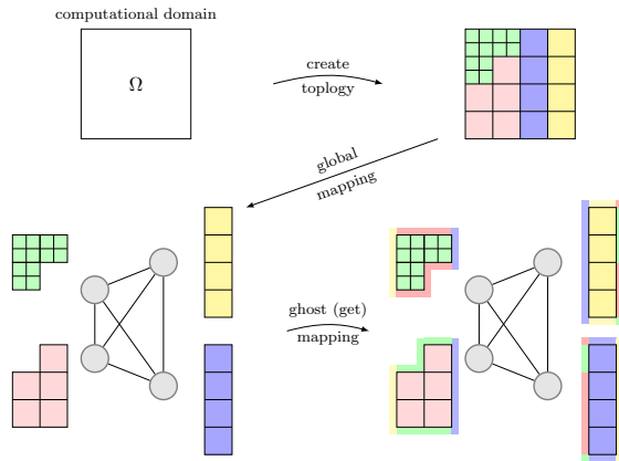
Figure 7.2. Using the topology abstraction, the computational domain \Omega is decomposed and the sub-domains assigned to processors (upper panels). The global mapping abstraction distributes particles, meshes, and connections across the processors (represented by the graph) as specified by the topology (lower-left panel). The ghost get mapping abstraction creates ghost layers around subdomains according to the topology and the boundary conditions (in the example shown here, periodic boundary conditions).
