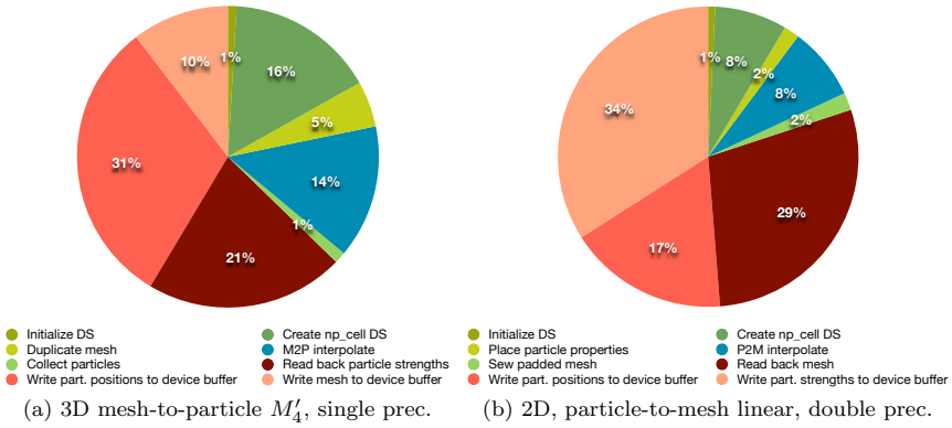
Figure 6.16. Breakdown of the computational time on the NVIDIA Tesla C2050 GPU by kernel. We show the case (a) that delivered the largest speedup, i.e., 3D mesh-to-particle interpolation using the M'_4 scheme in single precision and (b) the case that delivered the smallest speedup, i.e., 2D particle-to-mesh interpolation using the linear scheme in double precision.
