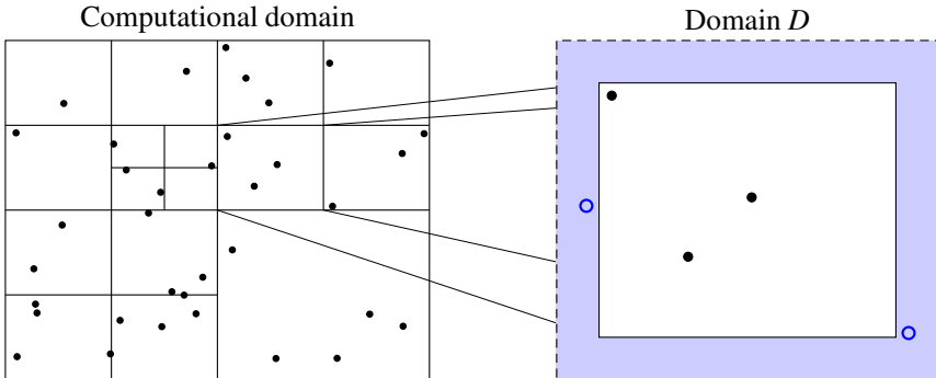
Figure 4.1. The computational domain is decomposed into cuboidal subdomains with halo layers (light blue). The halo layers contain ghost particles (blue circles) that are copies of real particles (black dots) from the adjacent subdomains. Independently applying the present algorithm to each extended subdomain (including the halo layers) D allows transparent implementation of boundary conditions and (distributed-memory) parallelism.
