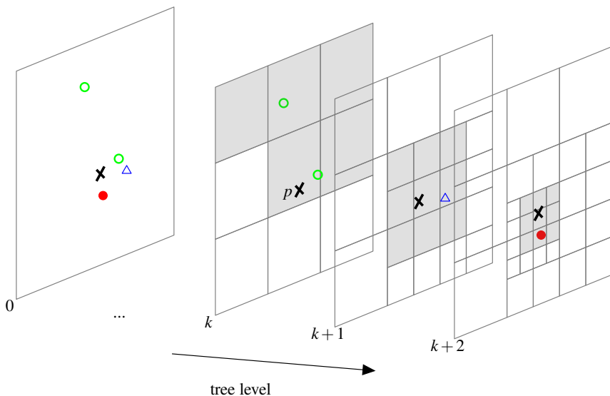
Figure 4.3. Finding interaction partners of a particle in an AR cell list (one iteration of Algorithm 4.3). The back plane (tree level 0) shows all particles without the cell-tree decomposition. In order to compute a symmetric interaction (or construct the Verlet list) of particle p (black cross) on level k we first iterate through all particles (green circles) in half of the neighboring cells \mathcal{N}(c_k) on the same tree level (shaded cells on level k ). Then, the finer tree levels are searched for interaction partners in the descendent cells c_k^\delta and their neighbors \mathcal{N}(c_k^\delta) (shaded cells on levels k+1 and k+2 ) on all finer levels \delta = k+1, \dots, \text{maxlevel} . On these finer levels, all neighboring cells must be visited in order to include all interaction pairs across different levels of resolution (blue triangles on level k+1 and red dots on level k+2 ). Transparent cells are not considered when computing this interaction.
