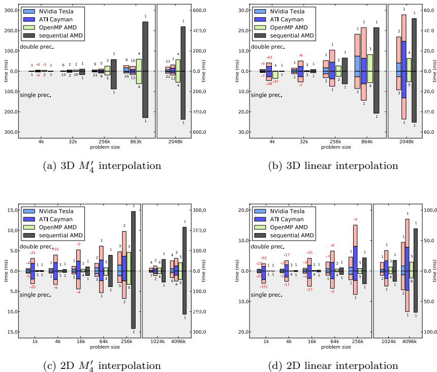
Figure 6.17. Timings for mesh-to-particle interpolation. We compare the wall-clock times of the OpenCL implementation run on the NVIDIA Tesla GPU (light-blue bars) and on the ATI Cayman GPU (dark-blue bars) with those of the Fortran90-OpenMP implementation running on an 8-core AMD FX 8150 CPU at 4.2GHz (8-thread: green bars, sequential: gray bars). The times needed to transfer the data to and from the GPU device memory are added in red. Bars pointing downwards refer to single-precision runs, bars pointing upwards to double-precision runs. The speedups with respect to the sequential CPU implementation are given above/below the bars. Speedups 1/x < 1 are given as -x in red. Notice the different time axes for the two parts of each plot. The CPU implementation does not make use of the processor’s vector units and therefor has similar runtimes for single-precision and double-precision runs.
