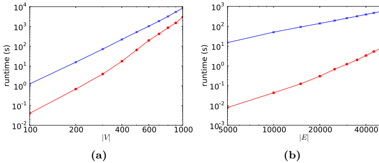
Figure 5.4. Runtimes of dsatur and vizing for graphs of increasing |V| and \deg(v) = |V|/2 \forall v \in V (a), and graphs with |V| = 1000 and increasing |E| = (|V|\deg(v))/2 (b). Both vizing and dsatur 's runtimes rapidly increase with increasing density of the graph.
