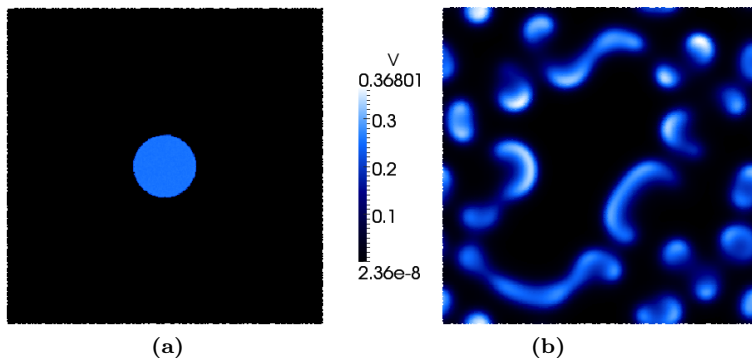
Figure 8.1. A PPML Gray-Scott reaction-diffusion particle simulation using the discretization-corrected PSE method [Schrader et al., 2010] with 10^5 particles. (a) Initial condition (b) concentration field of V after 4 \cdot 10^4 time steps.
