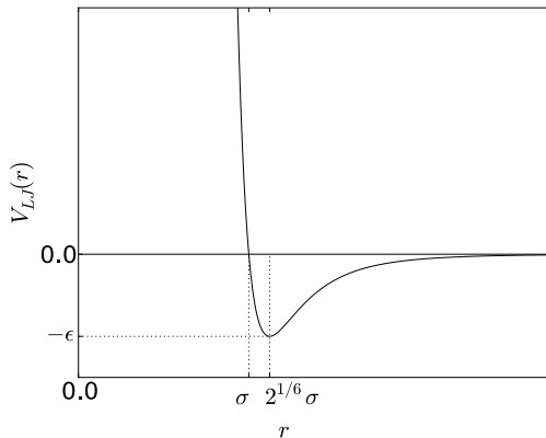
Figure 8.5. The Lennard-Jones potential function. \epsilon characterizes the depth of the potential well, while \sigma is the distance at which the potential is zero. The potential well's minimum can be found at 2^{1/6}\sigma .
