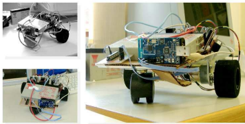
Figure 1: RAIN agent prototype layout.
