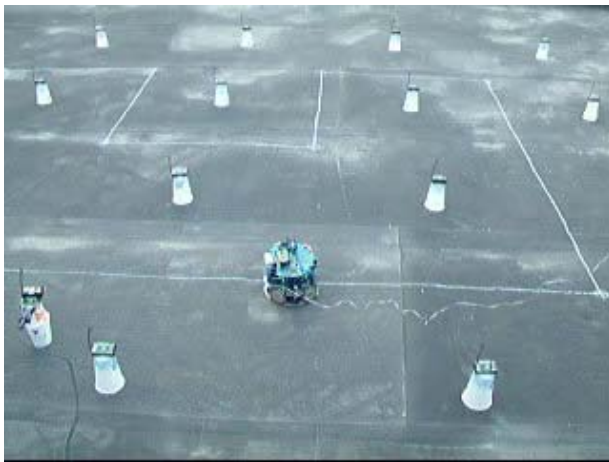
Fig. 1 The demo platform: 5×4 mika2 and a robot
