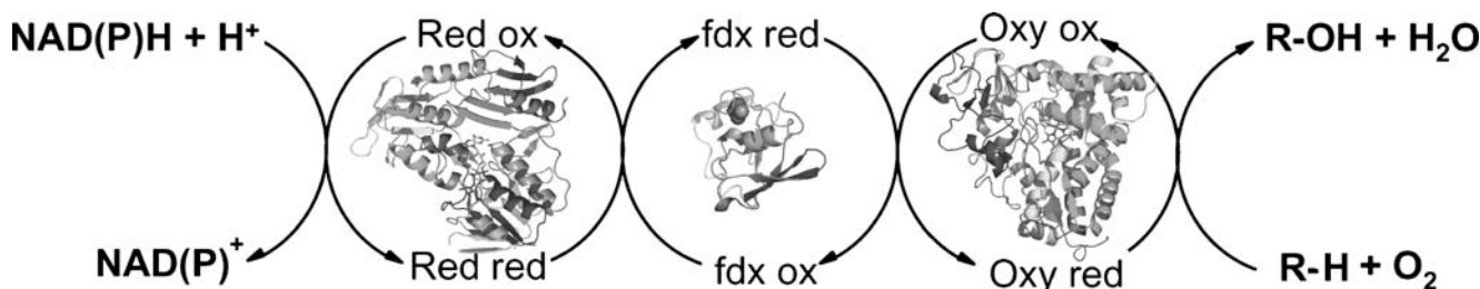
Fig. 2 Schematic representation of the various components of an alkane hydroxylase system and its electron transfer system. A reductase protein ( red ) transfers electrons from NAD(P)H via a small electron transfer protein ( fdx ) to the hydroxylase ( oxy ) protein where the substrate is oxidized to an alcohol, aldehyde, carboxylic acid, or
