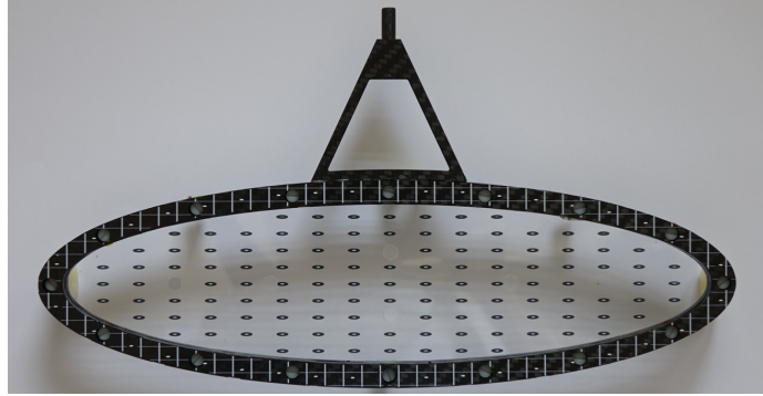
Figure 1.7: The MEG II target from [2]. A pattern of white dots on black background is printed on the scintillating foil and on the frame to monitor the position and possible deformation of the target through data taking.
