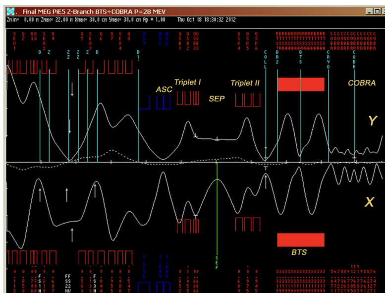
Figure 3.8: Second order envelope of the surface muon beam along the \pi E5 beamline in the MEG II configuration computed with TRANSPORT from [31]. Top: vertical envelope. Bottom: horizontal envelope. The dashed line represents the dispersion along the beamline in case of a momentum higher than nominal by 1%
