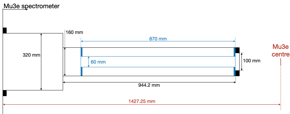
Figure 3.20: Sketch of the beam pipe and of the insert used for the commissioning at Mu3e center. The beam pipe has a diameter of 160 mm and an exit window with a diameter of 100 mm. The insert has a diameter of 60 mm.
