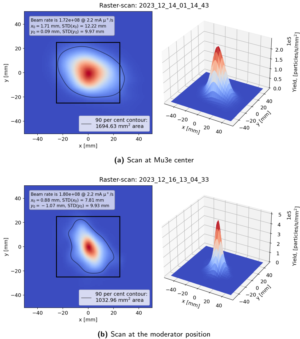
Figure 3.49: Raster-scan at Mu3e center (top) and at the moderator position (bottom) without beam pipe insert: the inner-most aperture of the beam pipe is 160 mm and the aperture of the exit window is 100 mm. To measure the beam spot at the moderator position, a 400 mm long section of the beam pipe was removed.
