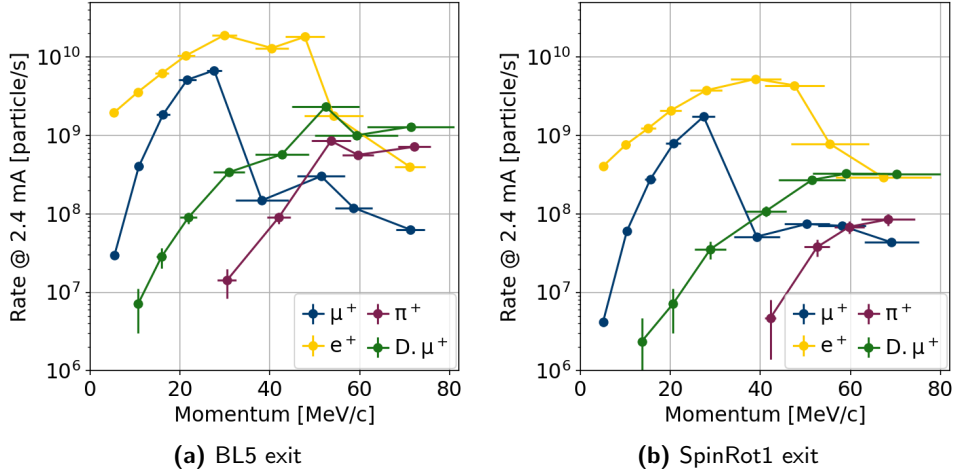
Figure 5.40: Maximum deliverable rate to the end of BL5 (left) and at the end of SpinRot1 (right) in MUH3. The rate was maximized for antimuons and computed for positrons and pions with the same tunes. SpinRot1 is off. Deep (D.) muons are shown in green. The error bars in the vertical direction are the statistical uncertainty on the computed rates. The error bars in the horizontal direction correspond to \pm 1 standard deviation of the transmitted momentum spectrum. Tunes lower than 30 MeV/c have been scaled down linearly from the surface muon tune.
