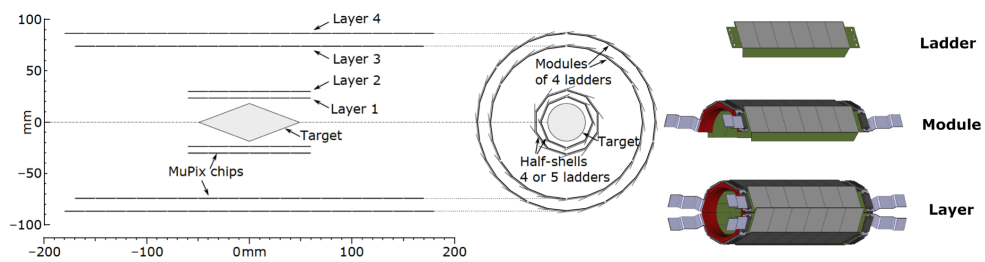
Figure 1.20: Left: geometry of the central tracker. Right: 3D-model of each sub-component of Layer 1. From [4].
