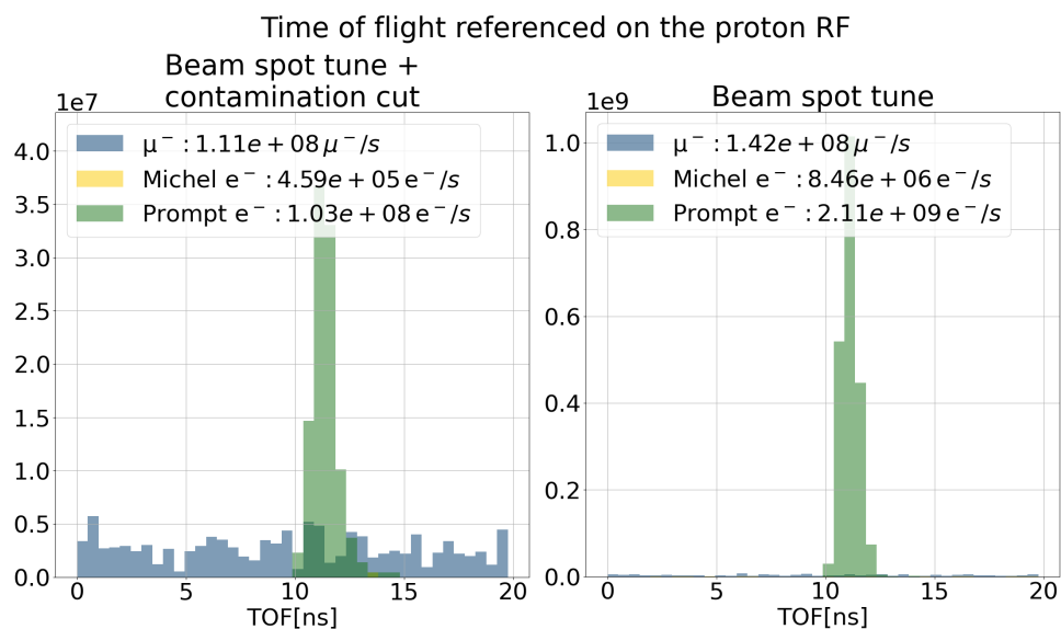
Figure 5.35: Spectrum of the time-of-flight modulo the period of the proton RF at the end of MUH2 for negative muon settings separated by type: negative muons in blue, Michel electrons in yellow and Prompt electrons in green. The distribution of negative muons is flat due to their large velocity spread at creation. Electrons are discriminated based on their creation time after proton interaction: Michel electrons are created after 5 ns; Prompt electrons are created within the first 5 ns. The scale does not represent the delivered rates. Left: beam spot tune with contamination cut. Right: beam spot tune.
