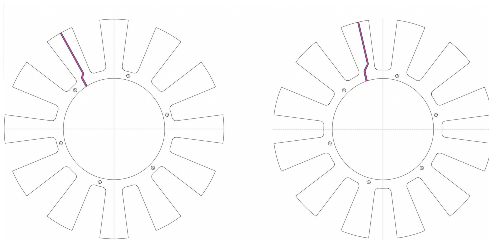
Figure 5.6: Schematic of the two disks composing TgH from [87]. Each disk has a thickness of 3.5 mm and sustains 12 blades. Once overlaid the two disks combine in a wheel. This design was preferred because it allows for a thicker graphite support at the center, where the disks overlap, without the need of machining a gradually varying thickness of the graphite. Additionally, it allows to precisely introduce gaps to keep distortions and thermal stress under control.
