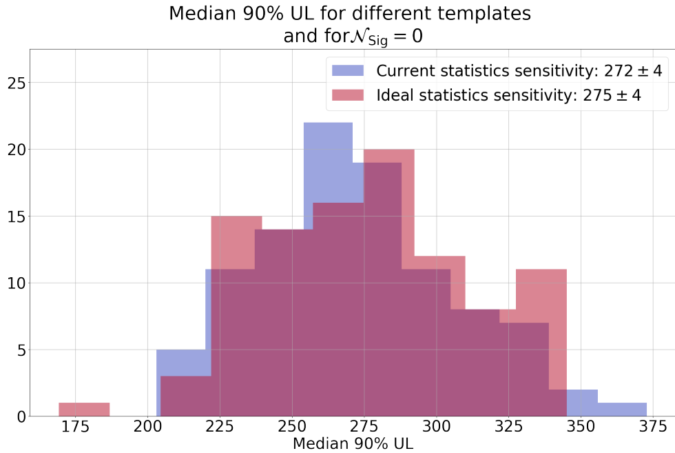
Figure 4.27: Distribution of the median 90% upper limit (UL) on the X17 yield for the ideal (red) and current (blue) statistics scenarios for \hat{N}_{\text{sig}} = 0 . Each point is computed by repeating the FC construction 100 times. A different template is used for each point. The sensitivity is quoted as the average of the medians of the upper limit obtained with the different templates. The quoted uncertainty is the standard deviation on the sample average.
