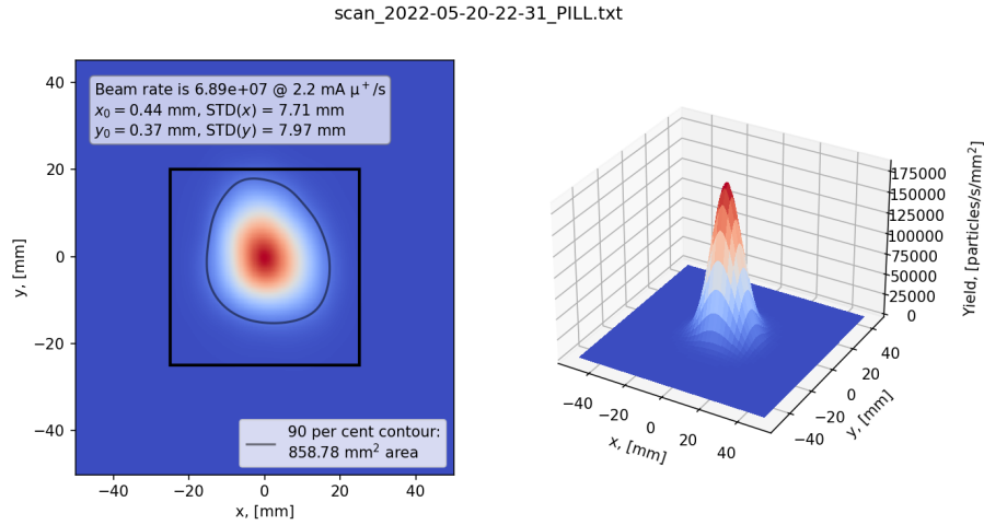
Figure 3.25: Raster-scan at Mu3e center including the beam pipe insert: the inner-most aperture of the beam pipe is 60 mm. The 40 mm aperture of the design vacuum window is included as well.
