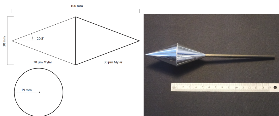
Figure 1.17: The Mu3e target from [4]. Left: a sketch of the Mu3e target. Right: a picture of the Mu3e target.
