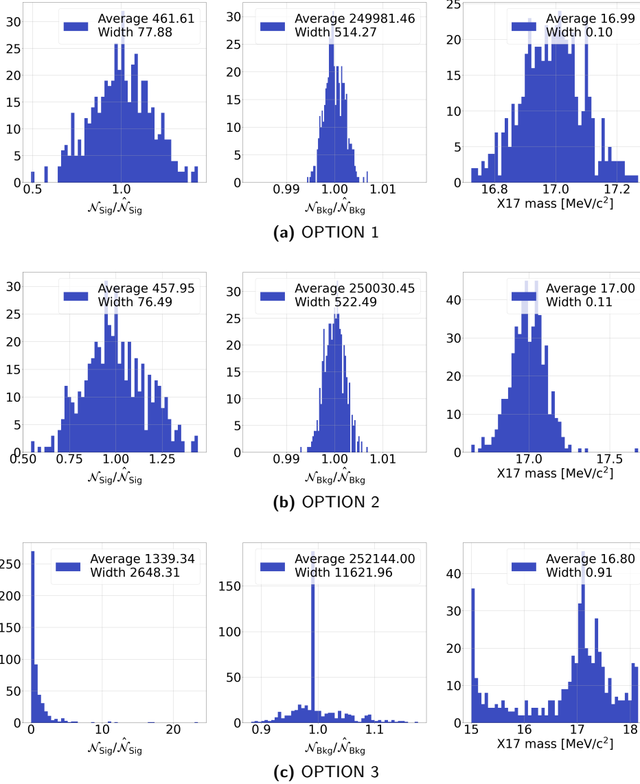
Figure 4.18: Distributions of the yield estimators and of the X17 mass estimator generated by fitting 500 different ToyMCs with the binned likelihood. The yields are normalized to their averages and the background yields are summed to improve readability. The effect of the nuisance parameters linked to the EPC PDFs is shown. OPTION 1 (top) and OPTION 2 (center) reported in Section 4.3.1 do not introduce changes with respect to the estimators in Figure 4.17. OPTION 3 (bottom) instead causes the estimated signal yield to be always compatible with zero. The overpopulated bin in the background yield is due to the minimizer reaching the limits of the allowed range for the signal parameters.
