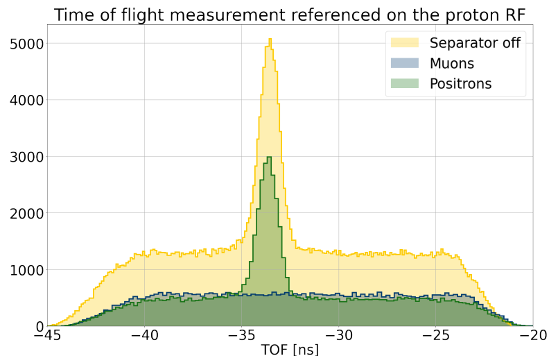
Figure 3.11: Time of flight spectrum measured at collimator for different separator settings: off (yellow), muons (blue) and positrons (green). The TOF is defined as the difference between the discriminated Pill signals and the RF-signal. The scale does not represent the delivered rates. The tails of the distributions are due to the finite resolution of the apparatus and to the time walk of the DRS4 evaluation board, which measures the time the signals exceed the threshold and not the time to reach a fraction of their maximum.
