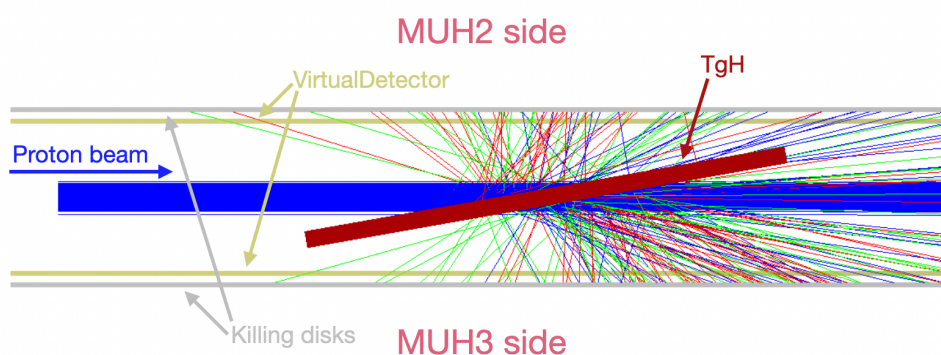
Figure 5.9: Zoom-in of the graphic output of the particle production at TgH from G4beamline. The target is seen from above. The secondary beams are produced by impinging 1000 protons (blue straight lines) on a simplified version of TgH (red). The particles are detected with two VirtualDetectors (light yellow) on the sides of the target and then absorbed by the two 'killing disks' (light grey).
