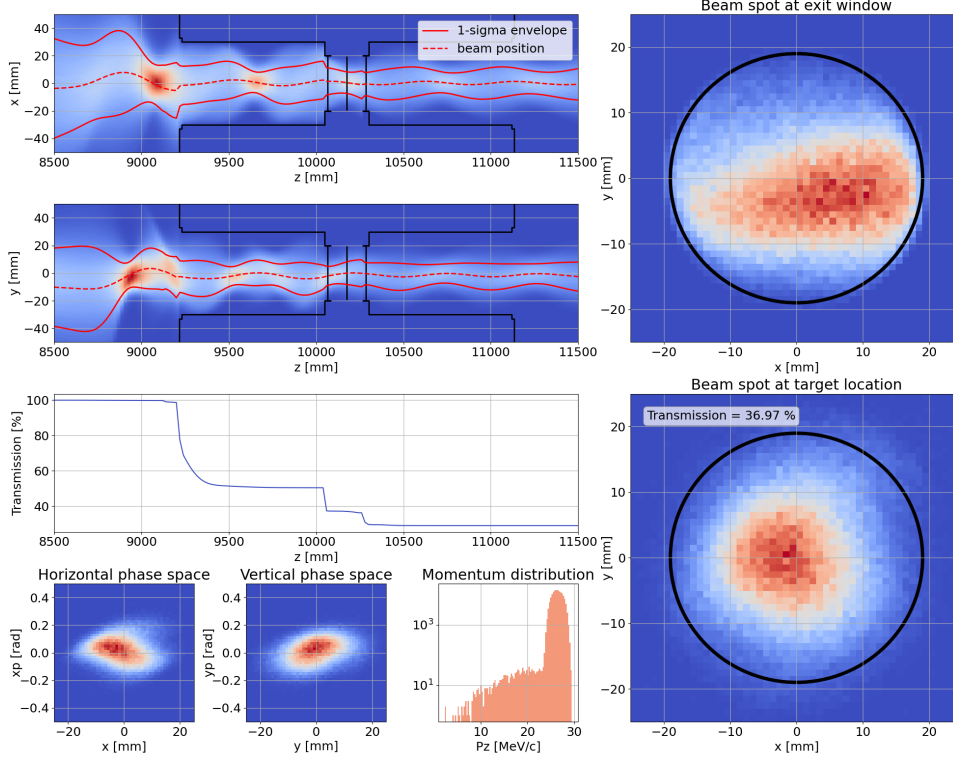
Figure 3.45: Transmission to the center of the Mu3e spectrometer. On the left from the top: the envelopes in the horizontal and vertical plane, the black lines show the size of the beam pipe; the transmission from the entrance of the magnet; the phase space at the center of the Mu3e magnet. On the right from the top: the beam spot at the vacuum window and the beam spot at target location. The black circles show the size of the target cross section.
