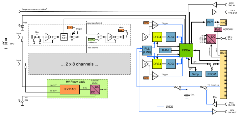
(a) WDB simplified schematics
