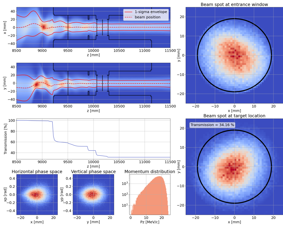
Figure C.3: Transmission to the center of the Mu3e spectrometer. The tune and the position of the moderator are optimized for 120% the nominal Mu3e spectrometer field value. The collimator position is optimized to minimize the muon rate on the inner layer of the Mu3e pixel tracker. On the left from the top: the envelopes in the horizontal and vertical plane, the black lines show the size of the beam pipe; the transmission from the entrance of the magnet; the phase space at the center of the Mu3e magnet. On the right from the top: the beam spot at the vacuum window and the beam spot at target location. The black circles show the size of the target cross section.
