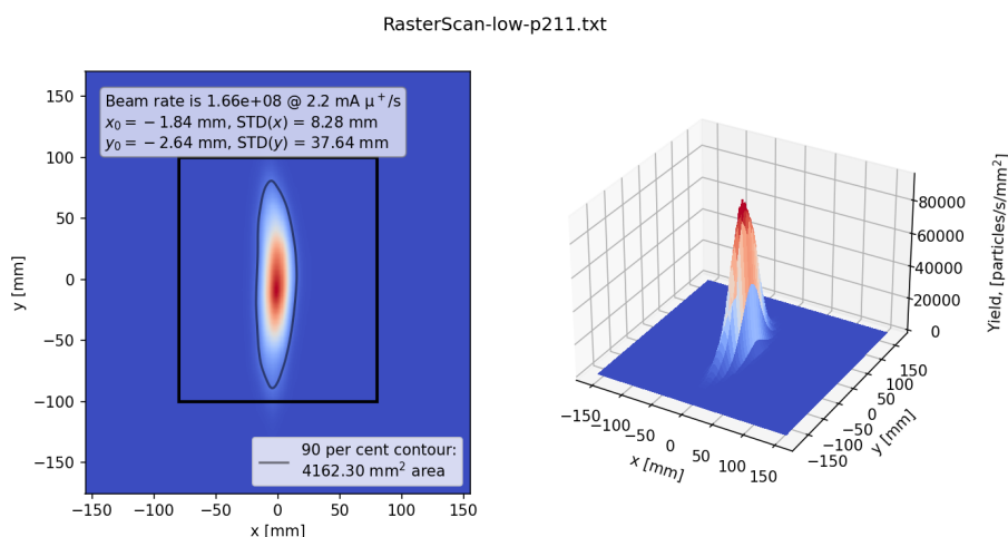
Figure 3.18: Raster-scan at QSM41. The currents are set to the optimum found at the end of the beam tuning. The black square on the left shows the region where the scan was performed, while outside of it the tails are estimated with a gaussian tail.
