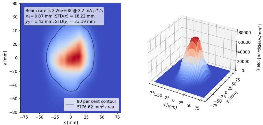
Figure 3.13: Raster-scan at collimator. The currents are set to the optimum found at the end of the beam tuning.
