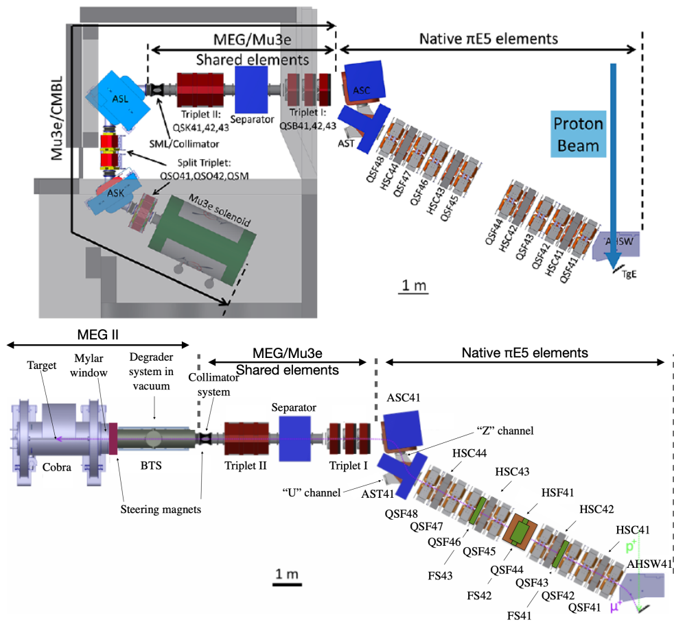
Figure 3.5: Top: \pi E5 layout in the Compact Muon BeamLine configuration from [4]. Bottom: \pi E5 layout in the MEG II configuration adapted from [2]. As reported above, the section up to the collimator is shared by MEG II and Mu3e. In CMBL configuration the front part of the area hosting Mu3e is separated by the rear part of the area hosting MEG II by a concrete wall positioned close to the ASL41 dipole.
