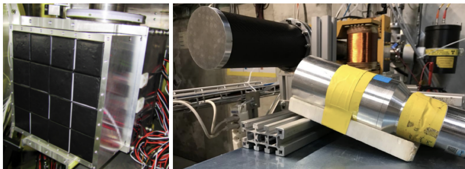
Figure 4.5: Auxiliary detectors used for the X17 measurement. Left: the 4 \times 4 BGO matrix used for the CEX measurement. Right: the 3-inch Brilliance crystal next to the carbon fiber vacuum chamber (black) for testing.
