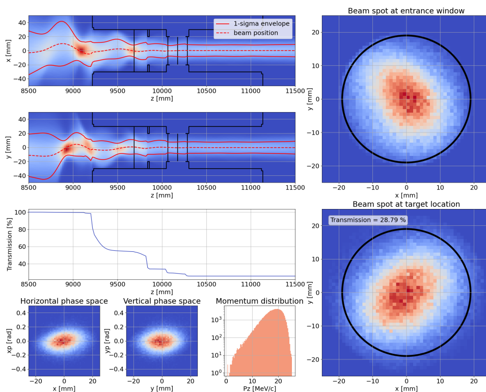
Figure C.1: Transmission to the center of the Mu3e spectrometer. The tune and the position of the moderator are optimized for the nominal Mu3e spectrometer field value. The collimator position is optimized to minimize the muon rate on the inner layer of the Mu3e pixel tracker. On the left from the top: the envelopes in the horizontal and vertical plane, the black lines show the size of the beam pipe; the transmission from the entrance of the magnet; the phase space at the center of the Mu3e magnet. On the right from the top: the beam spot at the vacuum window and the beam spot at target location. The black circles show the size of the target cross section.
