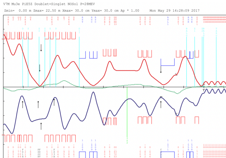
Figure 3.7: First order envelope of the surface muon beam along the \pi E5 beamline in the Mu3e configuration using the CMBL [5]. Top: vertical envelope. Bottom: horizontal envelope. The dashed green line represents the dispersion along the beamline in case of a momentum higher than nominal by 1%.
