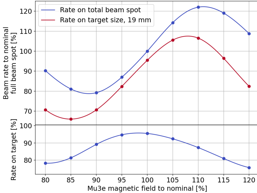
Figure 3.47: Top: the simulated rate estimated by integrating on the total beam spot (blue) and within the surface of the Mu3e target (red) at Mu3e center as a function of the magnetic field. Bottom: simulated fraction of beam within the area of the Mu3e target. The points represent the simulations. The solid lines are their interpolation with cubic splines.
