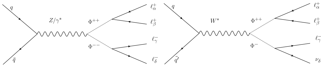
Fig. 1 Feynman diagrams for pair and associated production of \Phi^{++}
