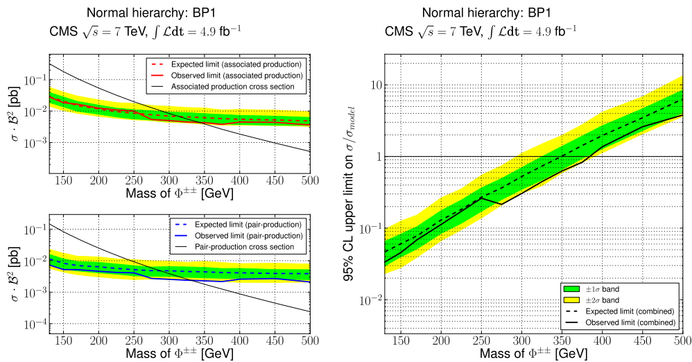
Fig. 11 Lower bound on \Phi^{++} mass at 95 % CL for BP1. On the left hand plots the B^2 means \mathcal{B}(\Phi^{++} \rightarrow \ell_\alpha^+ \ell_\beta^+) \mathcal{B}(\Phi^{++} \rightarrow \ell_\gamma^+ \ell_\delta^+) summed over all possible flavor combinations
