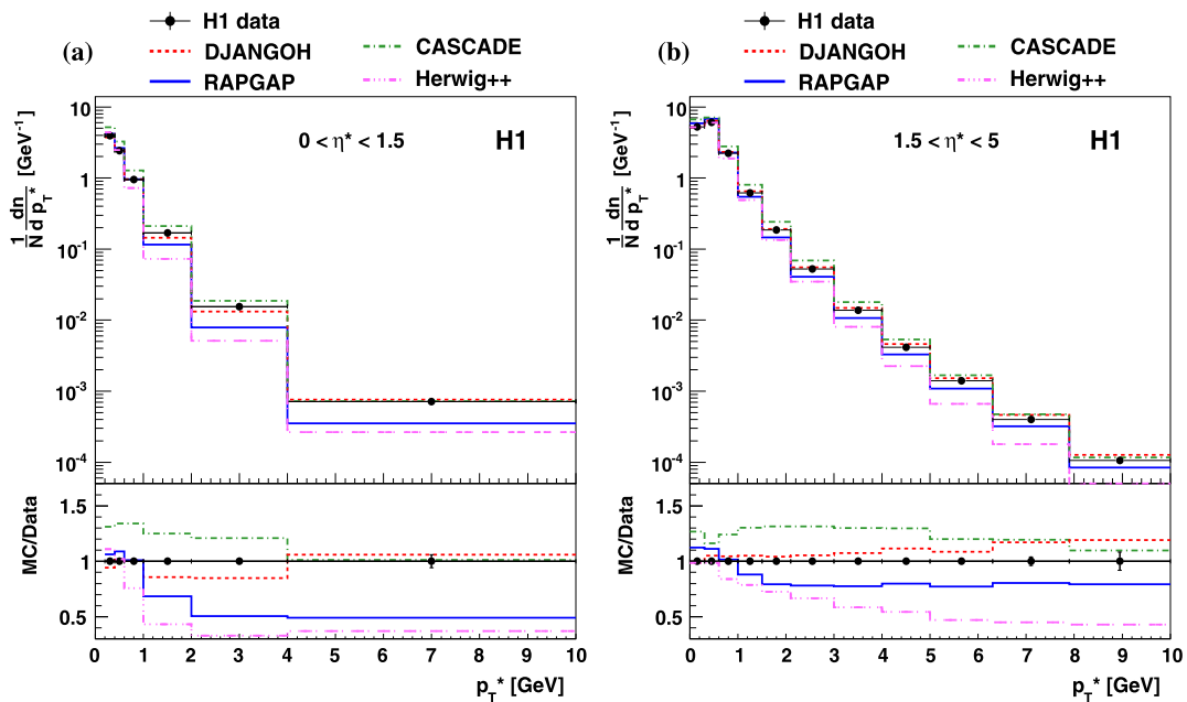
Fig. 8 Charged particle density as a function of p_T^* in the ranges (a) 0 < \eta^* < 1.5 and (b) 1.5 < \eta^* < 5 compared to DJANGO, RAPGAP, Herwig++ and CASCADE Monte Carlo predictions. The ratios of MC predictions to the measurements are shown on the bottom of the figure
