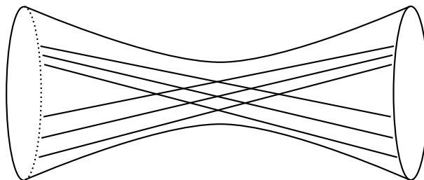
Figure 2. The coset SU(3)/(U(1) \times U(1)) can be represented as a quadric Q \subset \mathbb{C}\mathbb{P}^2 \times \mathbb{C}\mathbb{P}^2 . Two families of lines rule Q . Each line in the first family sits at a fixed point in the second \mathbb{C}\mathbb{P}^2 while each line in the second family sits at a fixed point in the first \mathbb{C}\mathbb{P}^2 . Since the \sim conjugation swaps the two \mathbb{C}\mathbb{P}^2 , it also interchanges the two families of lines. For lack of space we have not represented the X_3 submanifolds.
