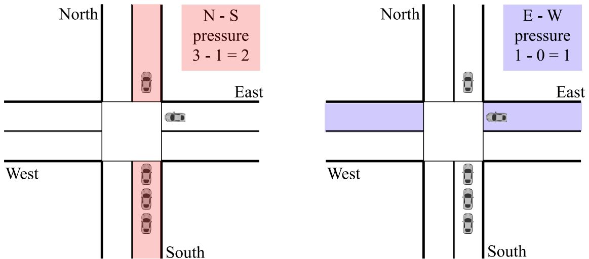
Fig. 2.3: Illustration of the max pressure control assuming we only have 2 possible movements, namely North-South and East-West, we can depict the pressure for each phase. In the current example, we see that the pressure for N-S is higher and thus would get activated in the next update. Here we assumed that c_{l,m} = 1 for all lanes.
