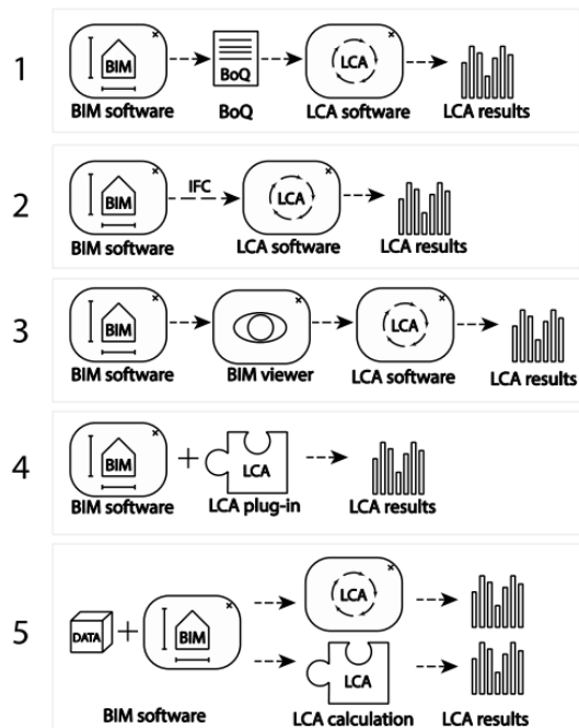
Figure 7: BIM-LCA integration types adapted from Wastiels and Decuyperre. Source:[8]
