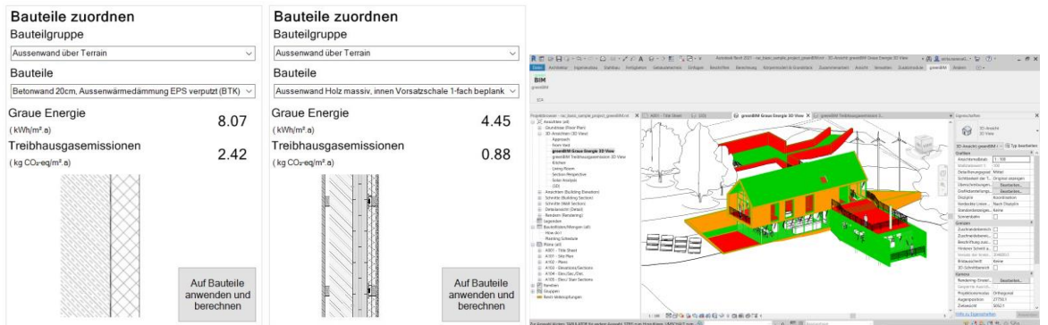
Fig 21: Components of the design (architectural model preliminary project) are linked with integrated components of the plug-in. Visualisations of LCA results in model.
