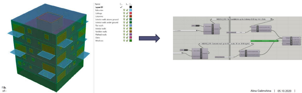
Figure 17: surfaces assigned to predefined layers and connected with grasshopper script. Source: Internal ETH
