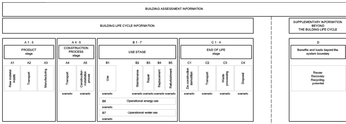
Figure 3: building life stages according to EN15978
