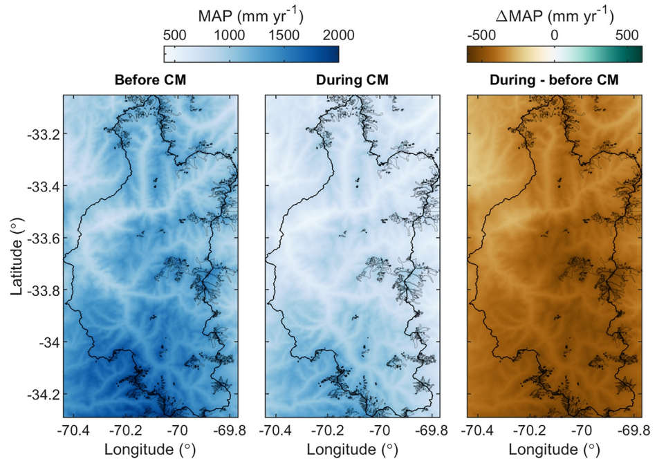
Figure 2. Mean annual precipitation (MAP) for the Maipo Basin at 0.005° spatial resolution, after downscaling and bias correction, for before (left) and during (middle) the current Chilean megadrought (CM). The rightmost panel shows the difference between the two periods. The basin is shown in black and the glaciers in gray.
