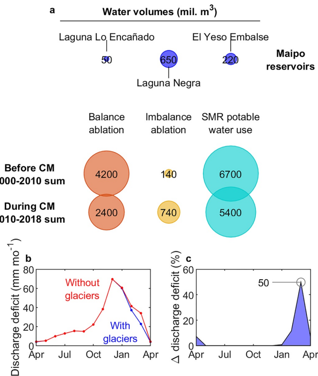
Figure 6. The importance of glacier runoff as a source of water. (a) Water volumes of Maipo Basin reservoirs at full capacity, balance and imbalance ablation sums for the before and during the current Chilean megadrought (CM) periods, and the potable water use of the Santiago Metropolitan Region (SMR) in these periods. (b) Comparison of the discharge deficits between before and during megadrought periods in the real world, with glaciers, and in a hypothetical world, without glaciers (i.e., without imbalance ablation). (c) The relative difference between with and without glaciers curves of panel (b).
