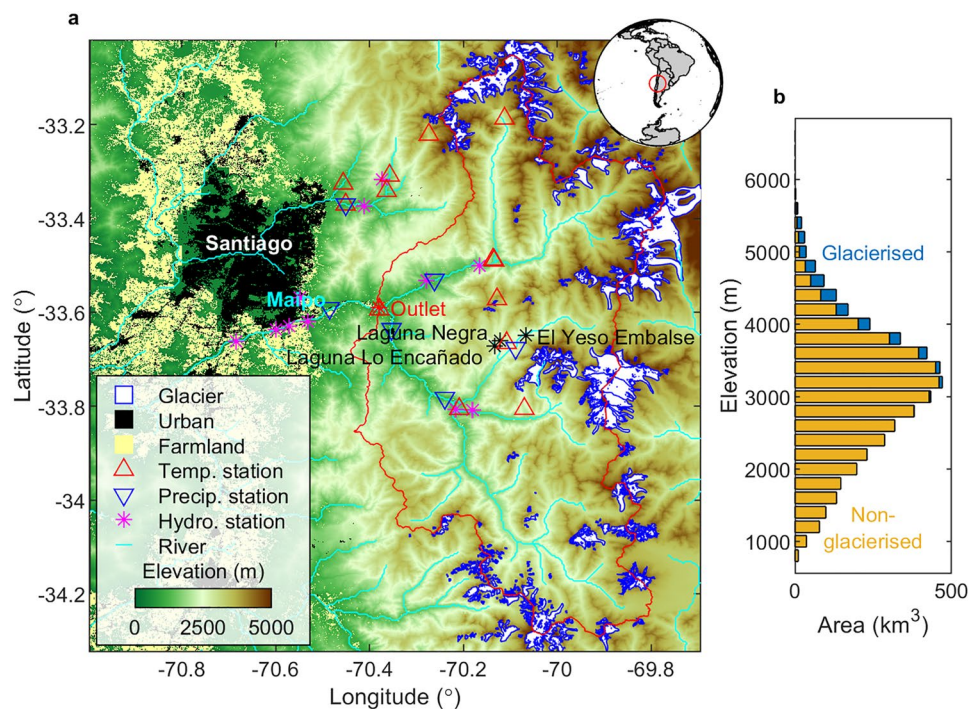
Figure 1. (a) The study area. The basin of the Maipo River in central Chile. The basin is outlined in red. The outlet is the Maipo El Manzano gauging station. Major reservoirs are marked with black stars. Glacier outlines are from RGI-Consortium (2017), urban areas are from Marconcini et al. (2020), and farmland is from Thenkabail et al. (2021). Temperature and precipitation stations are from Alvarez-Garretón et al. (2018). The elevation model is from JAXA (2019). (b) The basin's hypsometry.
