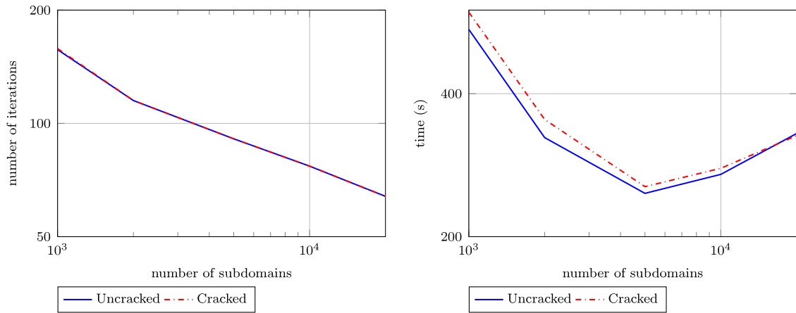
Fig. 18. Cracked compressor blade. Performance of deflation in conjunction to a block Jacobi preconditioner for the cracked and uncracked blade.
