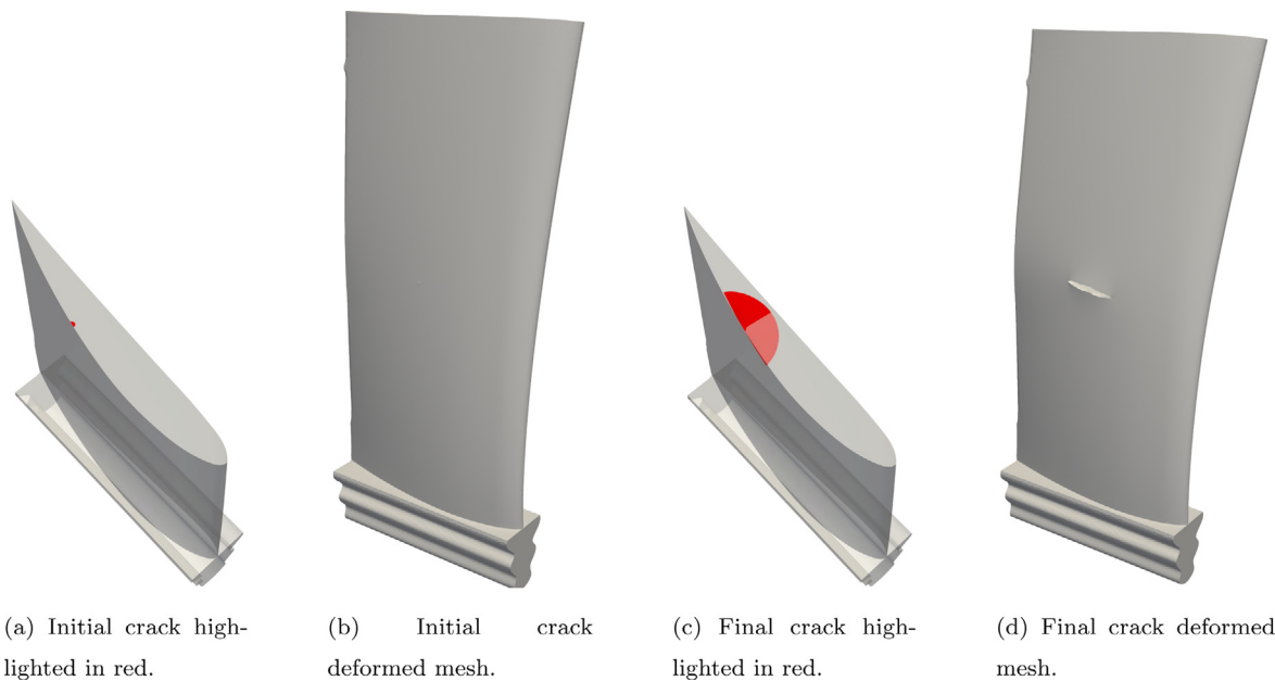
Fig. 19. Cracked compressor blade. Section with highlighted crack surface and deformed mesh for the initial and propagated crack after 60 steps of crack propagation. (For interpretation of the references to colour in this figure legend, the reader is referred to the web version of this article.)
