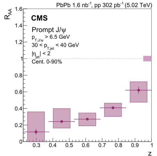
Fig. 5. Upper: The J/\psi differential cross section in pp and the T_{AA} -scaled yield in PbPb collisions, as a function of z . The normalization uncertainties of 1.9% for pp and 2.6% for PbPb are not included in the point-by-point uncertainty boxes and not shown in the plot. Lower: The nuclear modification factor R_{AA} , as a function of z . Bars indicate statistical uncertainties, while systematic uncertainties are depicted as boxes. The box around unity shows the normalization uncertainty.
