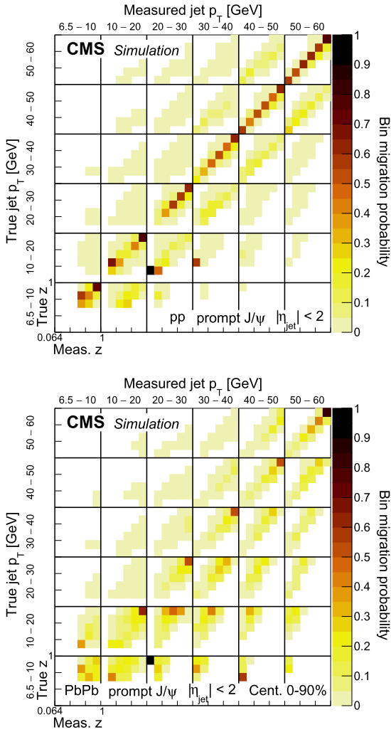
Fig. 2. Detector response matrices for jets containing a prompt J/\psi meson, showing the bin migration probability as a function of jet p_T and z . The response for pp collisions (upper) is evaluated using PYTHIA 8 . The response for PbPb collisions (lower) is evaluated using PYTHIA 8 embedded into HYDJET .
