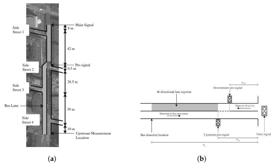
Figure 11. Layouts of presignals. Presignals turn red for cars when a bus arrives to it, irrespective of the main signal. That way buses can move through the intersection without encountering almost any traffic. (a) Layout of presignal in Zurich that changes lane allocation. Source: [24] (b) Layout of presignal that changes lane allocation and travel direction. Source: [78].
