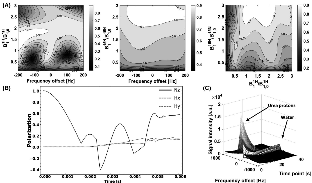
FIGURE 5 (A) Simulated efficiency of partial polarization transfer from ^{15}\text{N} to ^1\text{H} in [^{15}\text{N}_2]\text{urea} , defined as P_{\text{transferred}}/(1-P_{\text{preserved}}) . (B) Evolution of the ^1\text{H} and ^{15}\text{N} magnetizations. (C) Time course of polarization transfer from hyperpolarized ^{15}\text{N} to protons in a [^{15}\text{N}_2]\text{urea} phantom. The broad urea peak is the result of the degraded magnetic field homogeneity caused by injection of the hyperpolarized [^{15}\text{N}_2]\text{urea} solution. The residual water peak is the result of inadequate water suppression
