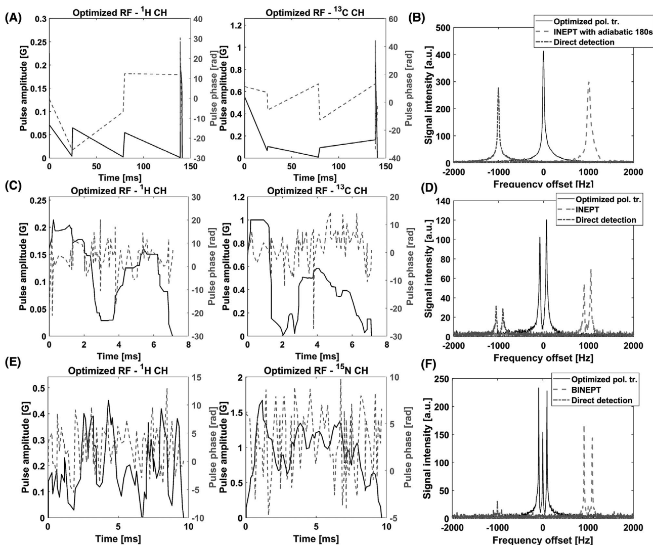
FIGURE 3 (A) Optimized pulses for transfer of {}^1\text{H} polarization to {}^{13\text{C}} in [1\text{-}^{13\text{C}}]\text{lactate} . (B) Comparison of the spectrum acquired with the optimized sequence to the spectra acquired with the adiabatic insensitive nuclei enhanced by polarization transfer (INEPT) sequence described in Ref. [14] and by detection without polarization transfer (direct {}^{13\text{C}} detection). The latter spectra are shifted by \pm 1000 Hz. (C) Optimized pulses for transfer of {}^1\text{H} polarization to {}^{13\text{C}} in [2\text{-}^{13\text{C}}]\text{lactate} . (D) Comparison of the spectrum acquired with the optimized sequence to that acquired without polarization transfer (direct {}^{13\text{C}} detection). (E) Optimized pulses for transfer of {}^1\text{H} polarization from the pairs of {}^1\text{H} nuclei to the {}^{15\text{N}} nuclei in [{}^{15\text{N}}]\text{urea} . (F) Comparison of the spectrum acquired with the optimized sequence to that acquired using the B_1 -insensitive heteronuclear adiabatic polarization transfer (BINEPT) sequence and by detection without polarization transfer (direct {}^{15\text{N}} detection). The latter spectra are shifted by \pm 1000 Hz
