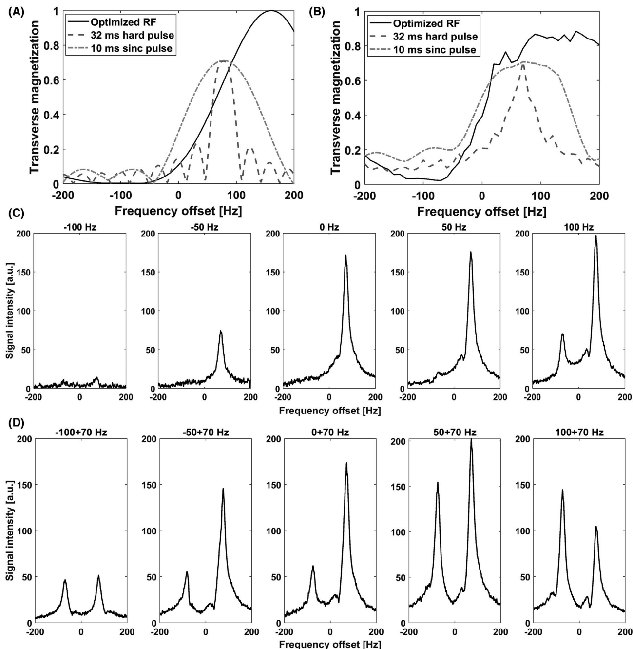
FIGURE 7 (A) Simulated frequency profile of the 9.76 ms optimized RF pulse designed to give J-coupling artefact-free excitation of [2- ^{13}\text{C} ]lactate when the pulse is applied exactly on-resonance at the center frequency of the ^{13}\text{C} doublet. The profile is compared to that of a +J/2 = 70 Hz off-resonant 32 ms hard pulse and a 10 ms sinc pulse. (B) The same profiles measured experimentally. (C) ^{13}\text{C} spectra acquired from [2- ^{13}\text{C} ]lactate with the optimized pulse at different offset values of the doublet center frequency. (D) ^{13}\text{C} spectra acquired from [2- ^{13}\text{C} ]lactate with the 10-ms sinc pulse applied at +70 Hz from different offset values of the doublet center frequency
