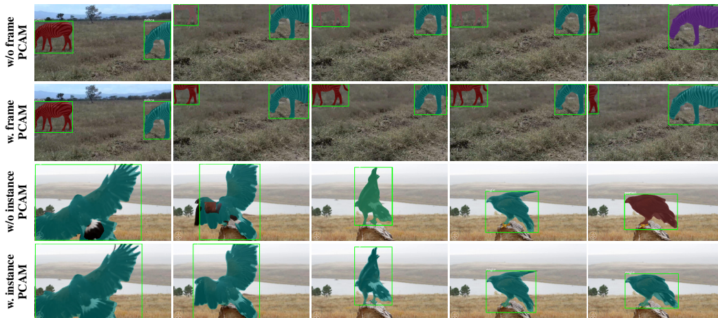
Figure 4: Qualitative impact of our PCAM on YouTube-VIS. Mask colors encode object identity. Our frame-level PCAM (second row) helps provide consistent detections and preserve identities compared to the baseline (first row). The instance-level PCAM (fourth row) provides more accurate masks, while further improving identity consistency compared to not employing our module (third row).
