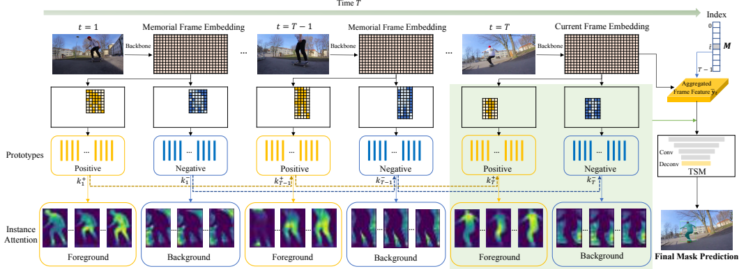
Figure 3: Our instance-level prototypical attention with foreground and background prototypes and temporal propagation. The foreground/background attention maps from (bottom) demonstrate the localized and discriminative appearance representation. Temporal Segmentation Module (TSM) takes the current frame, initial mask, and instance attention maps as input and generates the final mask.
