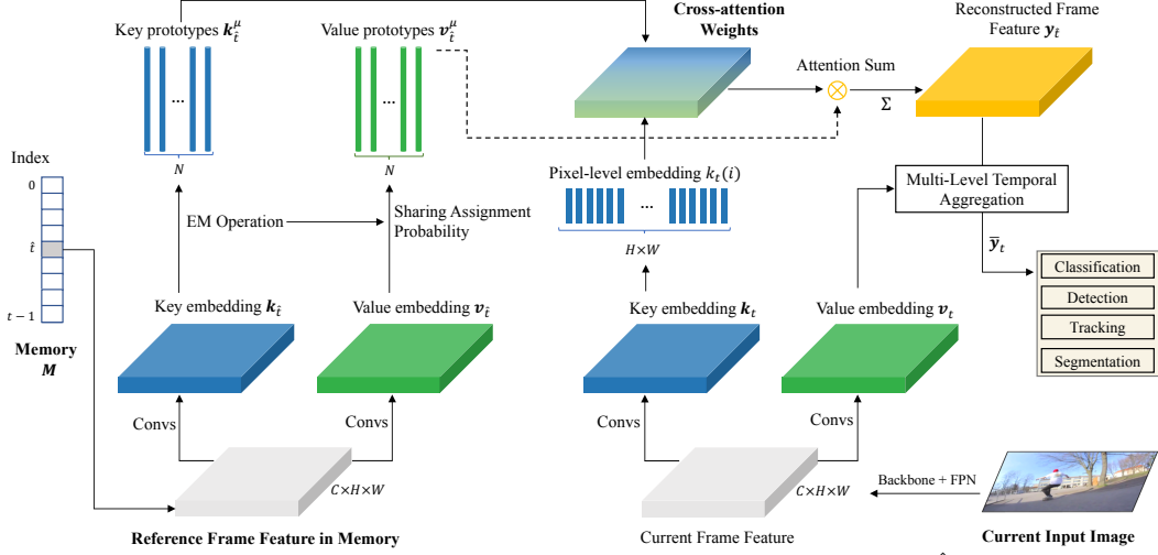
Figure 2: Overview of our frame-level prototypical cross-attention. For a frame \hat{t} in the memory we first perform GMM-based clustering to achieve the key \mathbf{k}_{\hat{t}j}^\mu and value \mathbf{v}_{\hat{t}j}^\mu prototypes. Given the key encoding \mathbf{k}_t of the current frame, we attend to the prototypes to generate the reconstructed feature \mathbf{y}_{\hat{t}} , which are then aggregated temporally and fused with the current value encoding \mathbf{v}_t .
