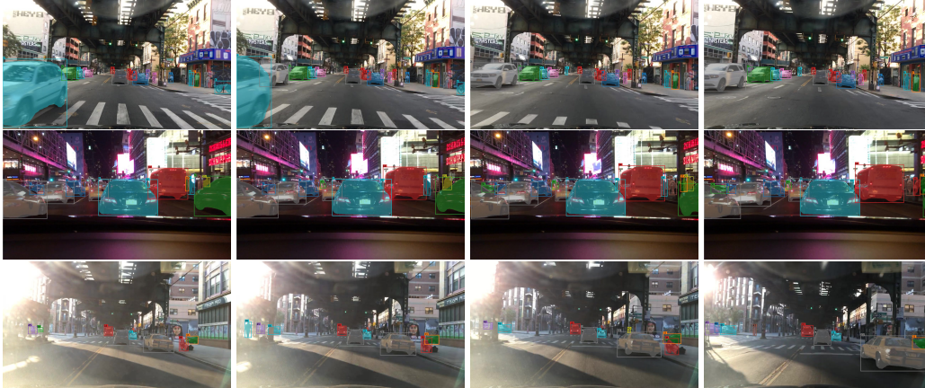
Figure 5: Qualitative results of our method on BDD100K. PCAN produces robust tracking and segmentation results under large motion and appearance changes (1st row) and heavy traffic in low-light conditions (2nd row). In the 3rd row, PCAN misses a detection (the person to the left in 1st frame), and produces tracking errors (2nd frame) when it covers totally different regions of the car with low appearance similarity. Zoom for better view. Video results are in the suppl. file.
