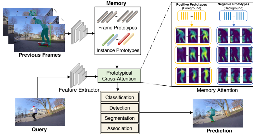
Figure 1: We propose Prototypical Cross-Attention Network for MOTs, which first condenses the space-time memory and high-resolution frame embeddings into frame-level and instance-level prototypes. These are then employed to retrieve rich temporal information from past frames by our efficient prototypical cross-attention operation.
