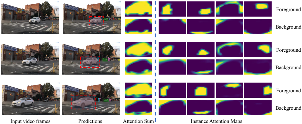
Figure 6: Instance cross-attention maps visualization for the car specified by the red dotted bounding box on BDD100K. We select the first four foreground/background prototypes as example, where each one focuses on specific car sub-regions with implicit unsupervised temporal consistency over time. proper technology management education, and having an open dialogue among various stakeholders on how such technology should be deployed and regulated.
