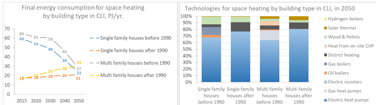
Figure 3.7: Total final energy consumption for space heating by type of building (left), and share of technologies supplying space heating in the different building types in the CLI scenario in 2050
