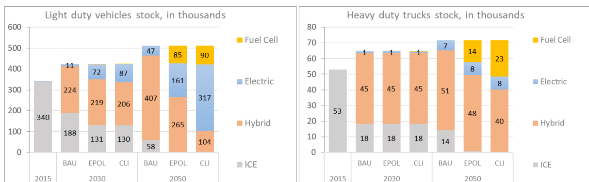
Figure 3.18: Composition of the stock of light-duty vehicles (left) and heavy-duty trucks (right)
