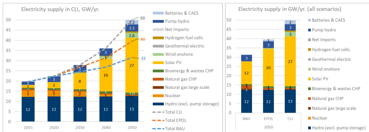
Figure 5.3: Trajectory of the electricity supply capacities, excluding the cross-border inter-connectors, in the CLI scenario (left), and comparison in 2050 across the three core scenarios (right)
