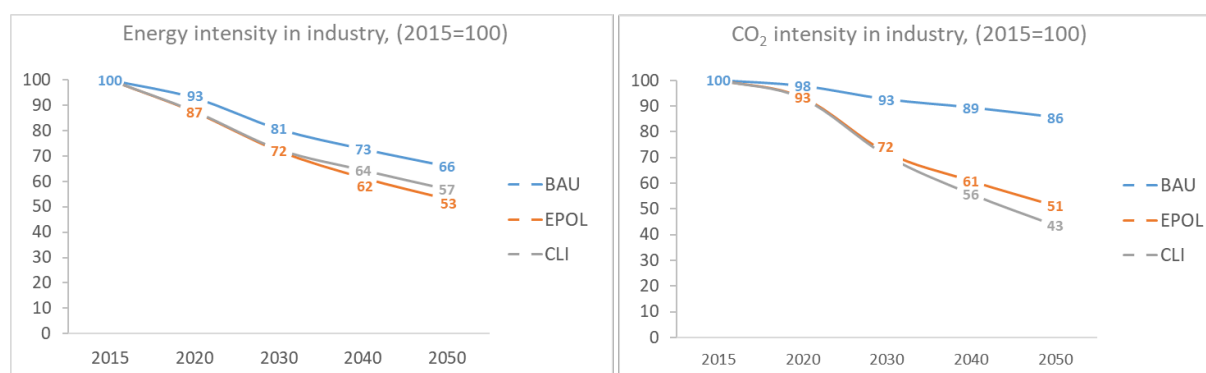
Figure 3.8: Improvement in energy intensity (unit of gross industrial value added produced per unit of energy consumed), and in CO 2 intensity (unit of emissions per unit of energy consumed)
