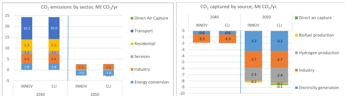
Figure 8.24: CO 2 emissions and CO 2 captured by sector; on-site CHP emissions are included in end-uses
