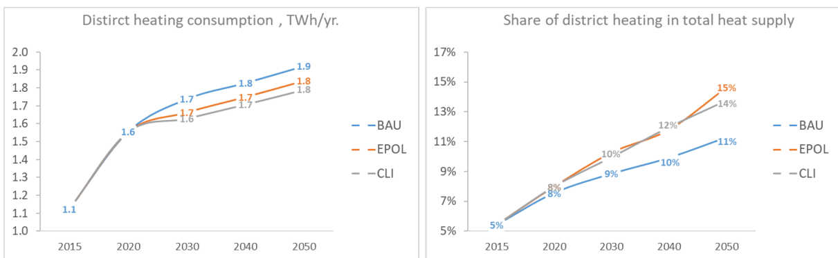
Figure 3.15: Consumption of heat from district heating networks in services (left) and share of district heating in total heat supply in the services sector (right)
