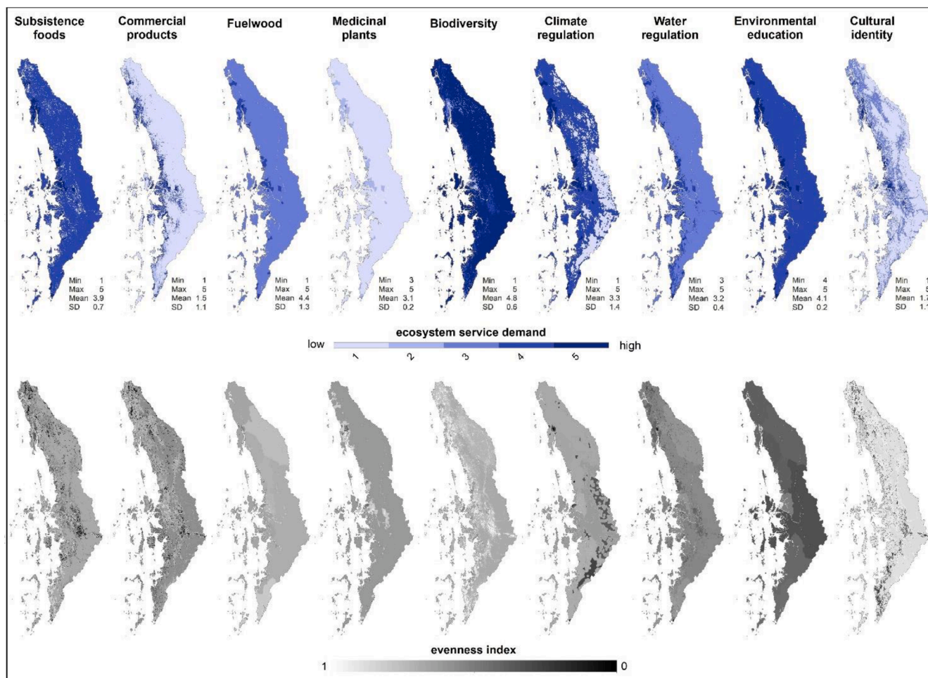
Fig. 3. Ecosystem service demand in Tanintharyi Region. Above : most likely ES demand values according to the models; below : corresponding evenness index representing uncertainty of those values (1 = maximum uncertainty, 0 = no uncertainty).
