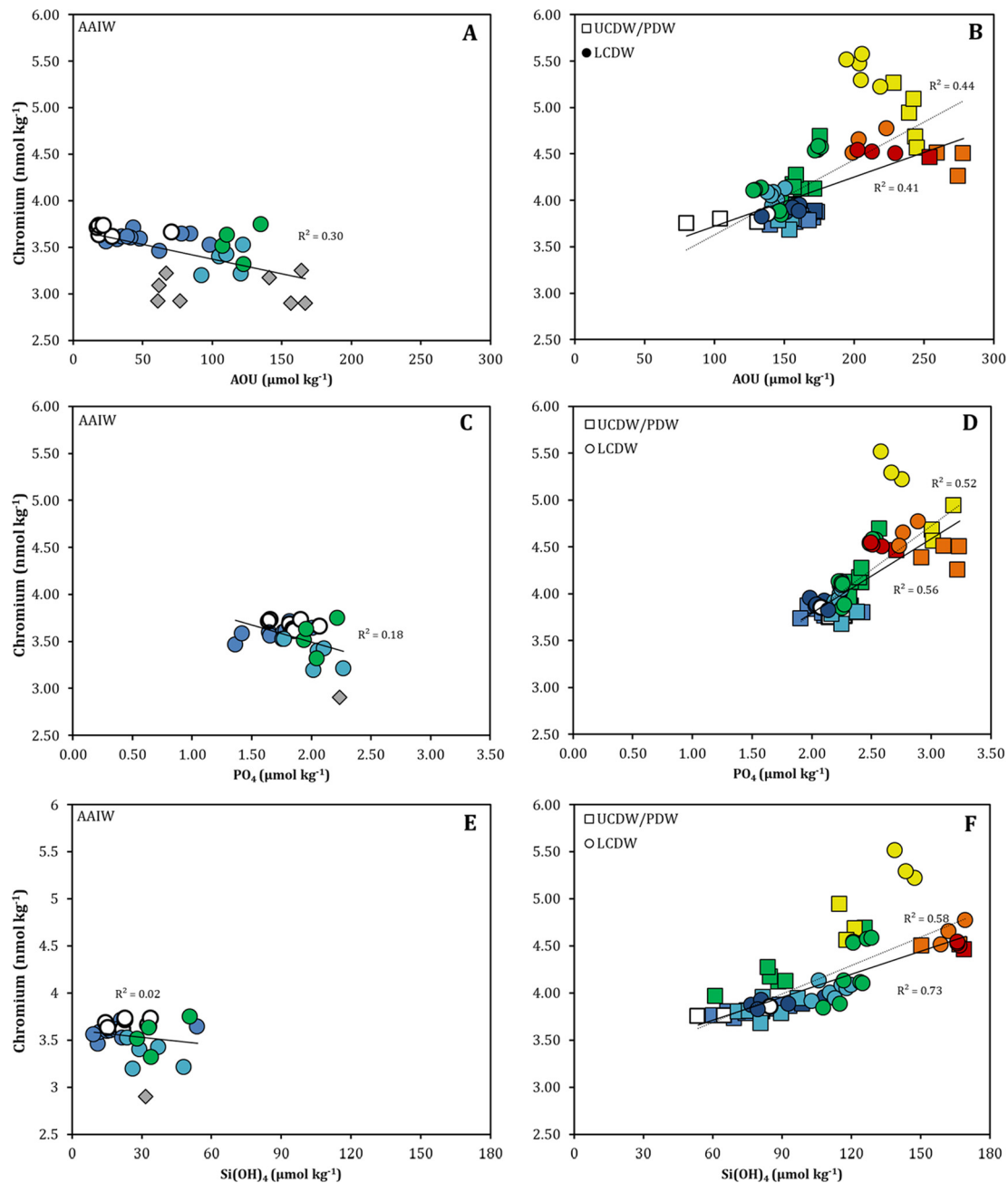
Fig. 5. Chromium–nutrient and Cr–AOU cross plots. Dissolved Cr is shown compared to AOU (A, B), \text{PO}_4 (C, D) and \text{Si}(\text{OH})_4 (E, F) for the intermediate (A, C, E) and deepwater (B, D, F) dataset to highlight decoupling of Cr from tracers of organic matter respiration and regeneration of organic-associated macronutrients (AOU, \text{PO}_4 ). Symbols follow those used in Fig. 4. Dashed lines in panels B, D and E indicate correlations across all data, while solid lines indicate correlations without ETSP data.
