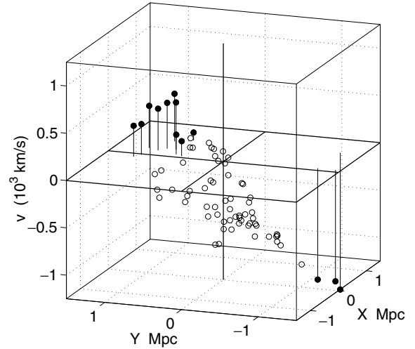
Figure 14. 3D Local Velocity Plot for Abell S333. This is Fig. A20(h) rotated counter-clockwise 50^{\circ} about the z -axis. This view clearly shows the spatial asymmetry in the local velocity with the northern half of the cluster (the leftmost two quadrants in the figure) moving away from the line of sight and with the southern half (the rightmost two quadrants) moving toward the line of sight.
