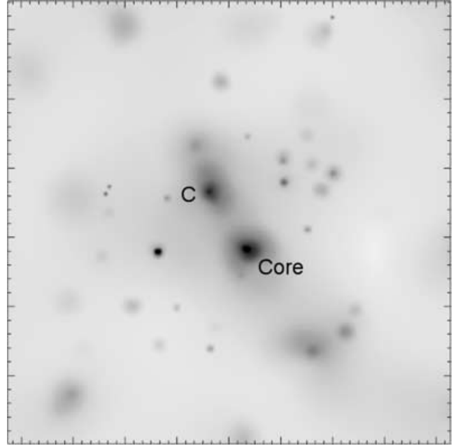
Figure 5. ROSAT PSPC image of Abell 1750 showing the two major components are associated with X-ray emission indicative of bound clumps. The brightest cluster member is located near the peak of the C subcluster emission.
