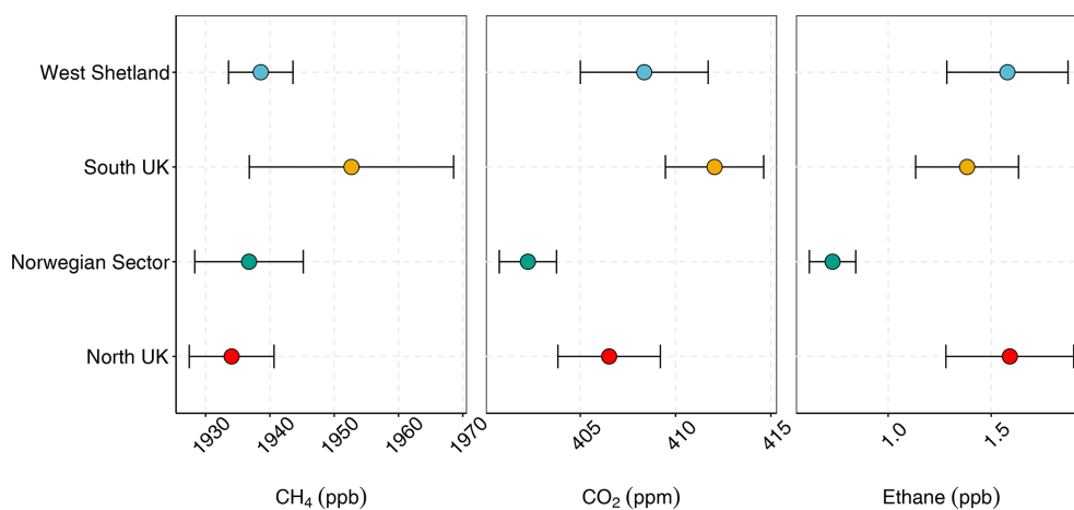
Figure A1. Mean background mixing ratios of CH 4 , CO 2 and ethane from all flights in each sampling region. Error bars represent 1 standard error.
