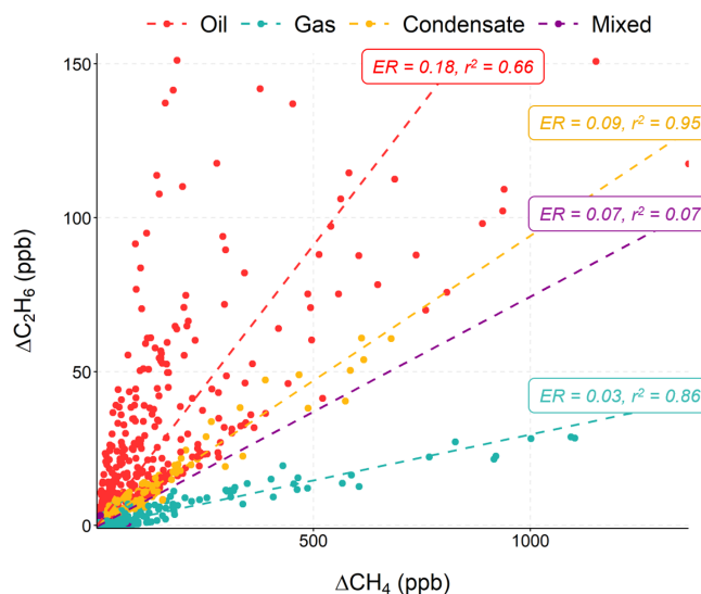
Figure 5. Scatter plot of \Delta C_2H_6 vs. \Delta CH_4 for each offshore field type. Observations were filtered to those with a \Delta CH_4 / \Delta CO_2 ratio greater than 20 \text{ ppb ppm}^{-1} as these were considered to be uninfluenced by anthropogenic urban emission sources. Dashed lines indicate the linear fit obtained from reduced major-axis regression.
