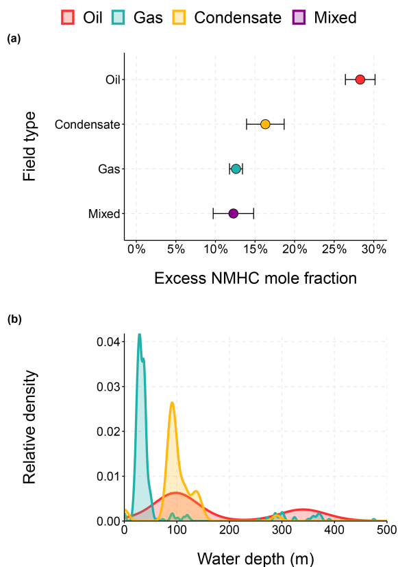
Figure 7. (a) Mean excess mole fraction for each offshore field type. Error bars represent 1 standard error. (b) Smoothed density distribution of water depth obtained for each offshore field in the North Sea, coloured by field type. A depth of 305 m (1000 ft) defines deepwater.
