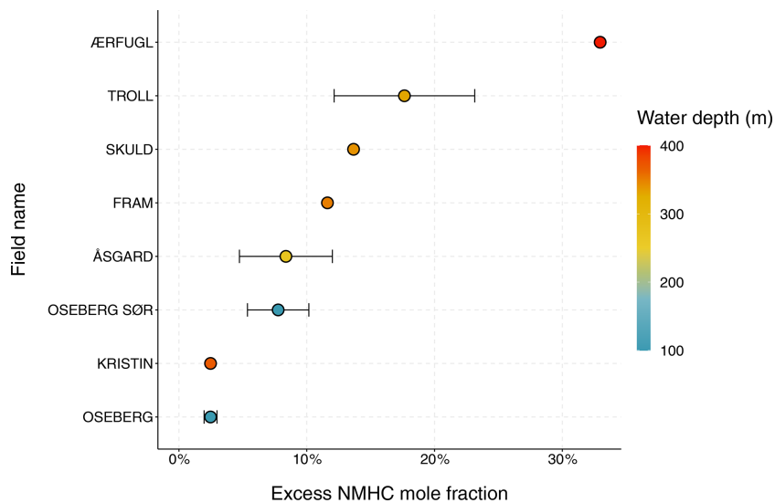
Figure A4. Mean excess mole fraction for individual offshore fields in the Norwegian sector of the North Sea coloured by water depth. Error bars represent 1 standard error.
