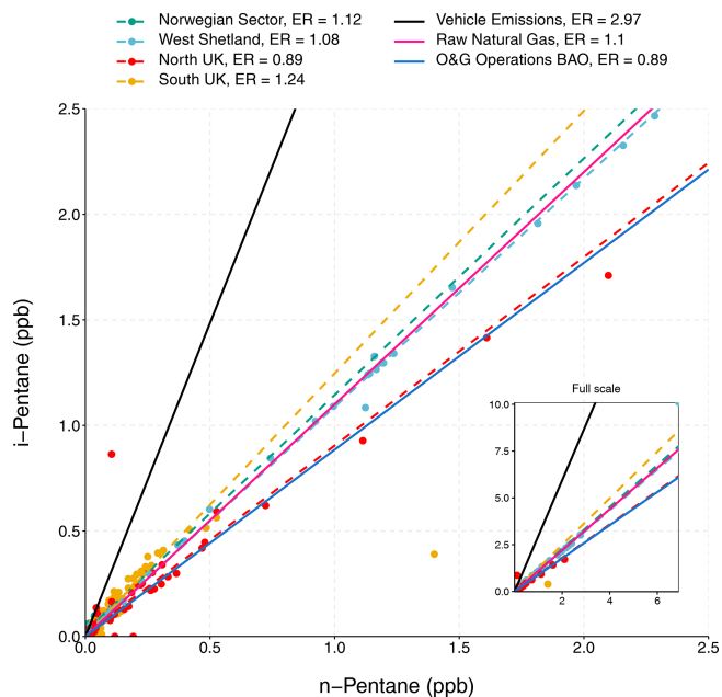
Figure 2. Scatter plot of iso-pentane and n -pentane observations in each sampling region. Dashed lines indicate the linear fit for each region obtained by reduced major-axis regression. The solid black line indicates the ratio from vehicular emissions (von Schneidmesser et al., 2010), the solid pink line shows the ratio of raw natural gas in the North Sea obtained from the Department for Business, Energy and Industrial Strategy (BEIS), and the solid blue line indicates a typical ratio from O&G emission sources (Gilman et al., 2013). Inset shows the full range of observations.
