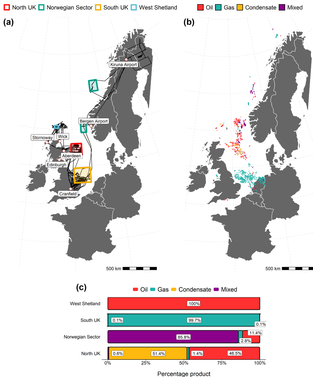
Figure 1. (a) Regions of the North Sea defined for analysis. The black lines represent the flight tracks of the research aircraft. (b) Location of all offshore fields in the North Sea. Each polygon is coloured by the extraction product from each field. (c) Percentage contribution of each offshore field type to the total area of all fields in each region. Country polygons were obtained using the “rnaturalearth” R package (South, 2017).
