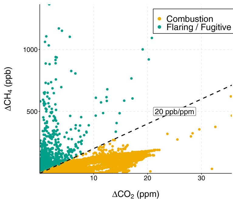
Figure A3. Scatter plot of \Delta\text{CH}_4 versus \Delta\text{CO}_2 . The dashed line shows an emission ratio of 20 \text{ ppb ppm}^{-1} , which was used for filtering data to remove the influence of anthropogenic emissions.
