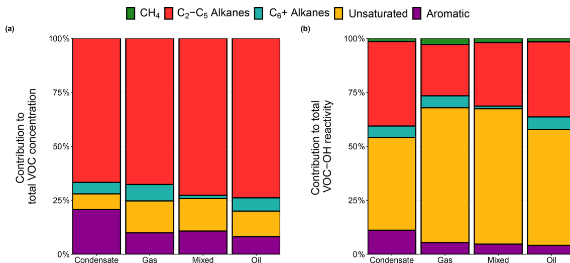
Figure 6. Percentage contribution of different VOC categories to (a) total VOC concentrations by mass and (b) total VOC-OH reactivity measured for each field type. The contribution of CH 4 is shown only for OH reactivity to demonstrate the relative importance of the other VOCs in terms of O 3 formation.
