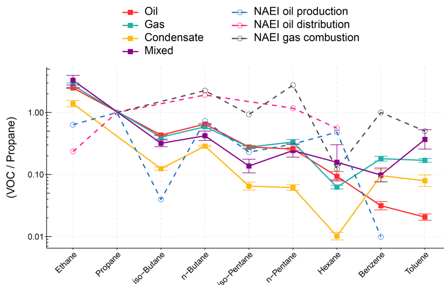
Figure 8. Emission ratios of VOC with propane calculated by reduced major-axis regression for each offshore field type (note the log scale). Error bars represent the 95 % confidence intervals. The dashed lines show the ratio obtained from the NAEI speciation profiles in Passant (2002) for oil production, oil distribution and gas combustion.
