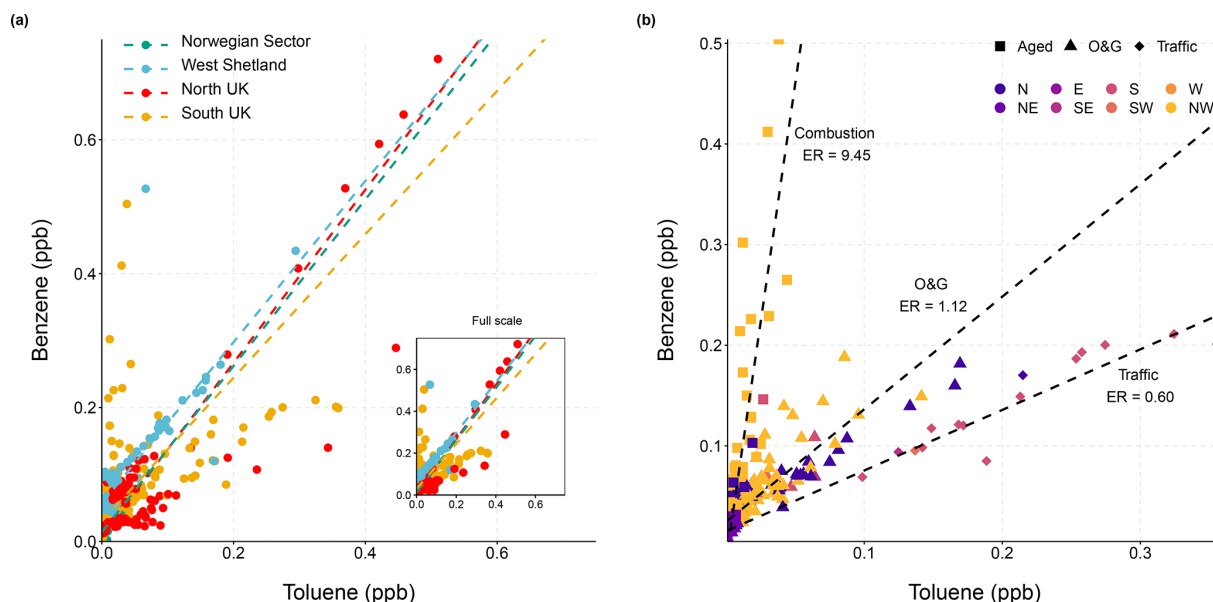
Figure 4. (a) Scatter plot of benzene versus toluene for all sampling regions. Inset shows the full scale of observations. (b) The southern UK only, where the colour represents the average wind sector during the time the sample was taken and the shape represents identified emission sources. In both figures the dashed lines indicate the linear fit obtained by reduced major-axis regression.
