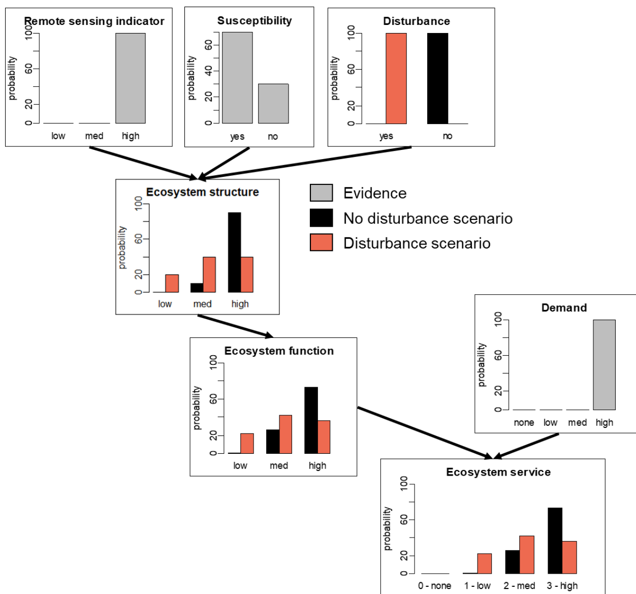
Figure 7.2: Conceptual representation of a Bayesian Network of an ecosystem service, where each box shows a node with its probability distribution over possible states. Evidence has been set for the nodes “Remote sensing indicator”, “Demand”, and “Susceptibility”, where the evidence for susceptibility is based on probabilities derived from modelling of natural disturbances in the region (Stritih et al., 2021). For the other nodes, the posterior probability distributions under a disturbance and no-disturbance scenario are shown. Risk related to disturbances is calculated as the difference between the expected values of the “Ecosystem service” node under the disturbance and no-disturbance scenario.
