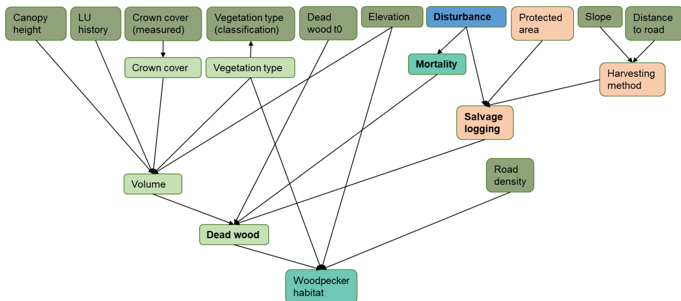
Figure D.3: Structure of the BN for habitat of the three-toed woodpecker. Nodes in bold are influenced by the disturbance BN.
