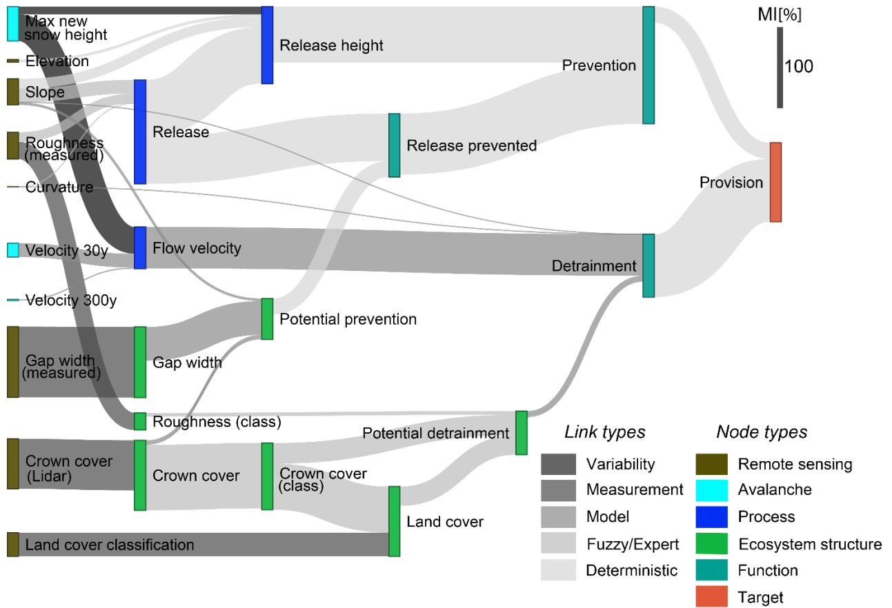
Figure 4.4: Stepwise sensitivity analysis of the BN, where the width of a link between two nodes corresponds to the relative mutual information (MI %), i.e. the percentage of the entropy on a node that can be reduced by a finding on a preceding node. The nodes are labelled and coloured by the type of variable represented (see Fig. 2), while the link colours represent the types of uncertainty taken into account while quantifying the link in the BN.
