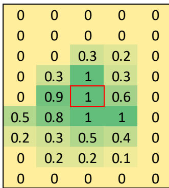
Figure B.2: Example raster of P(\text{release})
