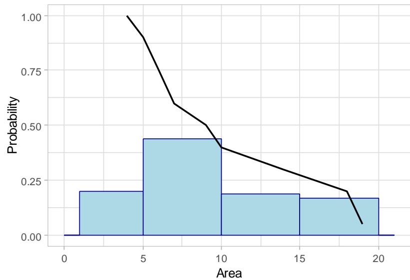
Figure B.3: Resulting cumulative probability distribution of area (black line) and the probability distribution of area in classes (1-5, 5-10, 10-15, 15-20 pixels).
