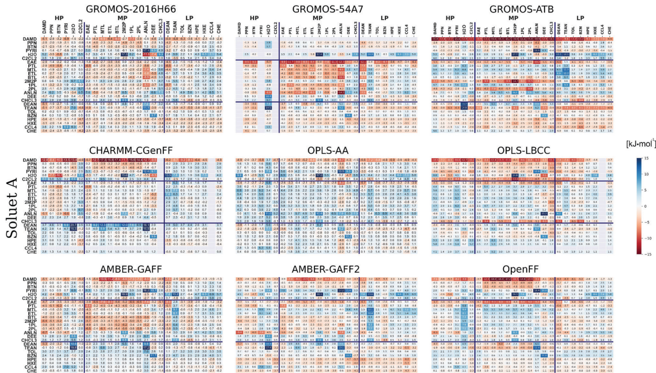
Fig. 5 Deviations between experimental and calculated cross-solvation free energies for the nine force fields considered. The \Delta_s G_{A:B}^{\ominus} deviations (calculation minus experiment) are given for the solutes A (rows) in the solvents B (columns). The force fields considered are listed in Table 1. The molecules considered and their acronyms are shown in Fig. 1. They are listed along the rows and columns in order of decreasing polarity, as estimated by the molecular dipole moment \mu , and the partitioning into low (LP), medium (MP), and high (HP) polarity categories is also indicated (see Fig. 1). The corresponding numerical values can be found in Section S8 of ref. 43 along with Section S1 (Table S3, ESI † ) of the present article. The calculated solvation free energies, their electrostatic components and their van der Waals components are displayed in Fig. S1–S3 (ESI † ), respectively.
