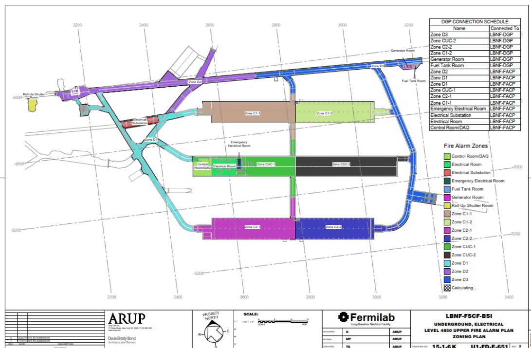
Figure 5.3. Underground fire zones.
