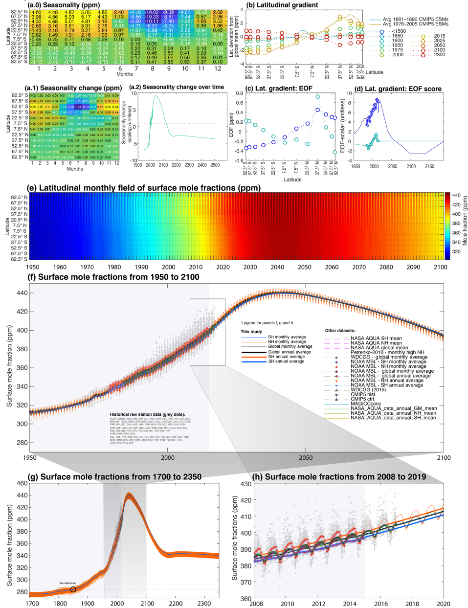
Figure 5. CO 2 concentrations under the SSP1-1.9 scenario. The base seasonality pattern derived from historical observations with monthly and 15° latitudinal resolution (a) is modulated over time using the first EOF of the residuals (a.1), scaled with projected NPP into the future (a.2). The latitudinal gradient is assumed to be flat in pre-industrial times, with latitudinal gradients over the observational record being derived from historical observations – and here compared with CMIP5 ESM models – see Meinshausen et al. (2017) (b). The projection of the latitudinal gradient uses global total CO 2 emissions regressed against the score (dark-blue line in panel d) of the first latitudinal EOF (dark-blue line in panel c). The principal component’s score of the second EOF’s is assumed to be zero in the future (turquoise line in panel c, d). Resulting surface air mole fraction fields show a return to current CO 2 (~ 2019) concentrations by the end of the 21st century (e, f). Historical NOAA surface flask station datasets (grey dots in panels f, g, h with station indicators provided in legend of panel f) are used for these future projections beyond the end of 2014 reach of the historical dataset (grey shaded background in panels f, g, h). Various comparison datasets shown, namely the WDCGG time series (Tsutsumi et al., 2009), the NOAA Marine Boundary Layer (MBL) product ( https://www.esrl.noaa.gov/gmd/ccgg/mb/ , last access: 20 June 2020) and the NASA AQUA satellite data ( ftp://acdisc.gsfc.nasa.gov/ftp/data/s4pa/Aqua_AIRS_Level3/AIRX3C2M.005/ , last access: 20 June 2020), the Petrenko time series (made available in the Supplement to Buizert et al., 2012). Also shown are the MAGICC global-mean projections (bright blue line “MAGICCconc”). These overview figures are available for all 43 gases and all nine scenarios on http://greenhousegases.science.unimelb.edu.au as a total of 387 so-called fact sheets. See also Table 12 in Meinshausen et al. (2017) for a description of all data labels.
