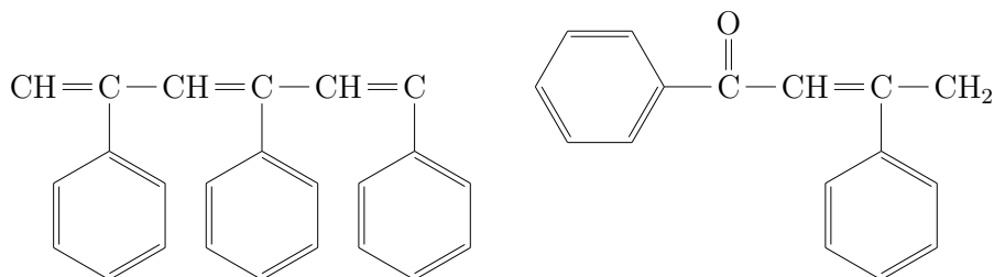
Figure 2. Examples of changes to polystyrene undergoing irradiation. The change on the right can only occur in the presence of oxygen.
