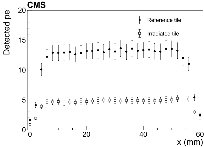
Figure 19. Number of detected photoelectrons for an SCSN-81 tile before and after an irradiation dose of 30 kGy at R of 9 Gy/h, as a function of the position of a radioactive-scan source along an axis through the center of the tile and parallel to one of its sides. The error bars are dominated by systematic uncertainty in normalization of the measurements; statistical point uncertainties are <2\% .
