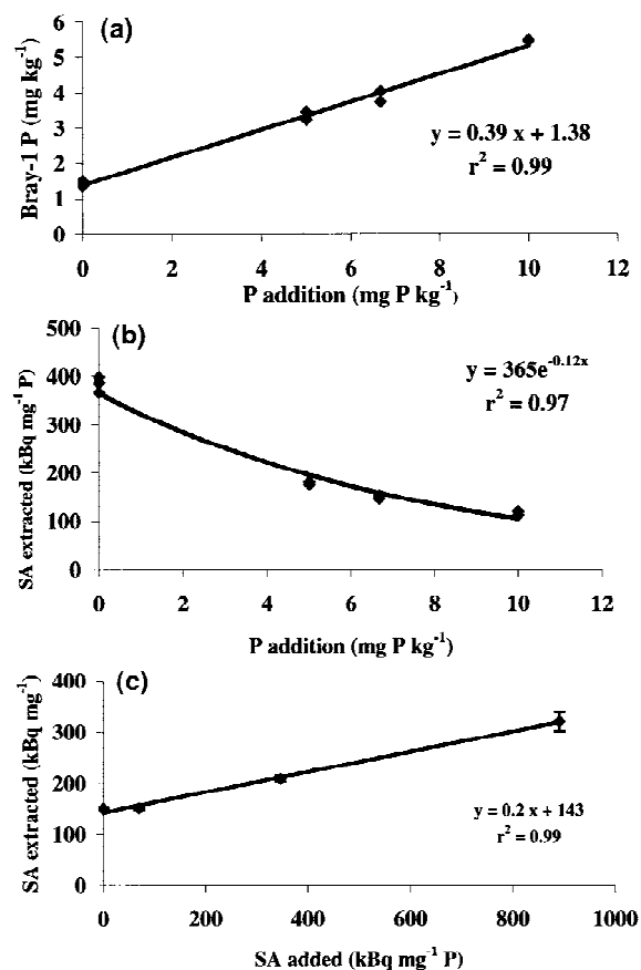
Figure 1. (a) Amounts of P extracted using Bray-1 as a function of the amount of unlabeled P added to the GL soil. Three (0 and 5 mg P kg -1 soil) or two analytical replicates per P addition. (b) Specific activity (SA) of Bray-1 extracted P as a function of the amount of unlabeled P added to the GL soil 2 days after labeling. Three (0 and 5 \mu g P/g soil) or two analytical replicates per P addition. (c) Specific activity (SA) of Bray-1 extracted P as a function of the SA of a constant amount of P (6.67 mg P kg -1 ) added with increasing ^{33}P activities to the GL soil 2 days after labeling. Each point presents a mean of three analytical replicates.
