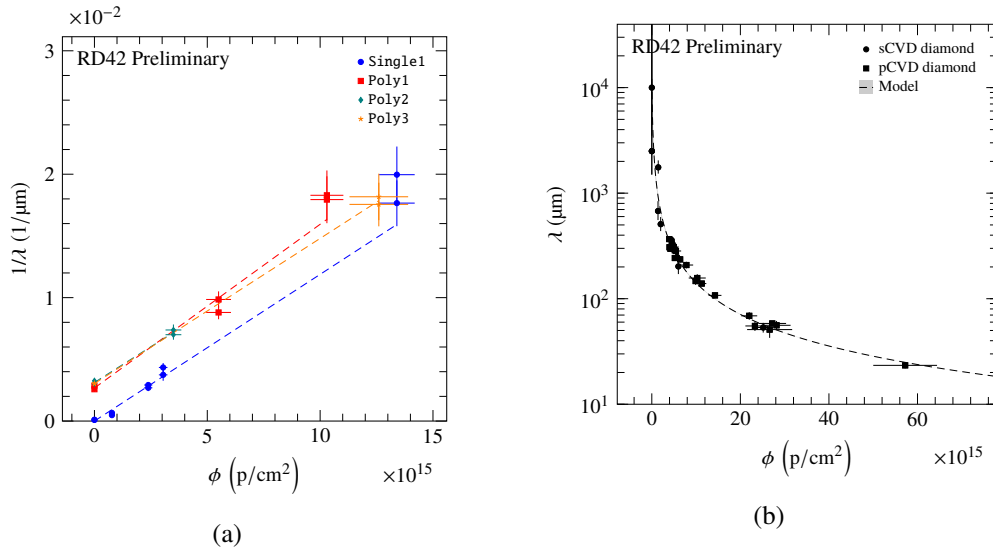
Figure 2: Measurements of inverse Schubweg as a function of 800 MeV protons fluence for sCVD and pCVD samples for two polarities with statistical and systematic error added in quadrature [3] (a). Measured Schubweg as a function of 24 GeV protons equivalent fluence compared to the radiation damage model (dashed curve) [3] (b).
