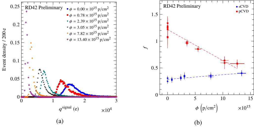
Figure 1: MIP signal spectra of single crystal diamond detectors at different 800 MeV proton fluences (a), and ratio of FWHM to the most probable value of the MIP signal for single crystal and polycrystalline CVD diamond (b) [3].
