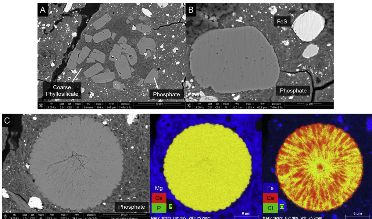
Fig. 8. BSE images of phosphate grains (a) associated with a coarse-grained phyllosilicate clast, and (b) in the matrix of Y-980115; (c) BSE image (left) and corresponding EDS maps showing the distribution of Mg (B), Ca (R), and P (G) (middle), and Fe (B) and Cl (R) (right) in a phosphate grain within Y-82162.
