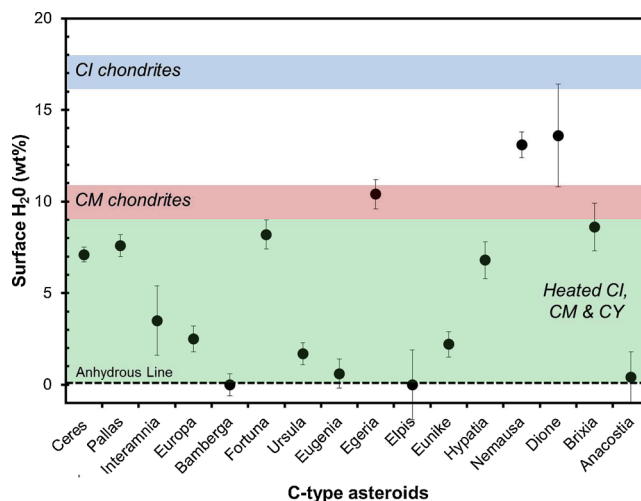
Fig. 14. Estimated H 2 O abundances for C-type asteroid surfaces compared to unheated and heated CI, CM and CY carbonaceous chondrites. Asteroid data are from Rivkin et al. (2003), and meteorite data are from Alexander et al. (2013); Garenne et al. (2014), and King et al. (2015b).
