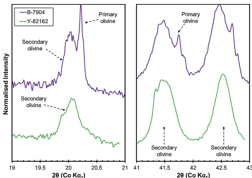
Fig. A1. XRD patterns highlighting the presence of crystalline primary olivine in B-7904. The patterns were collected using a PANalytical X'Pert Pro scanning XRD and Co Kα 1 radiation.
