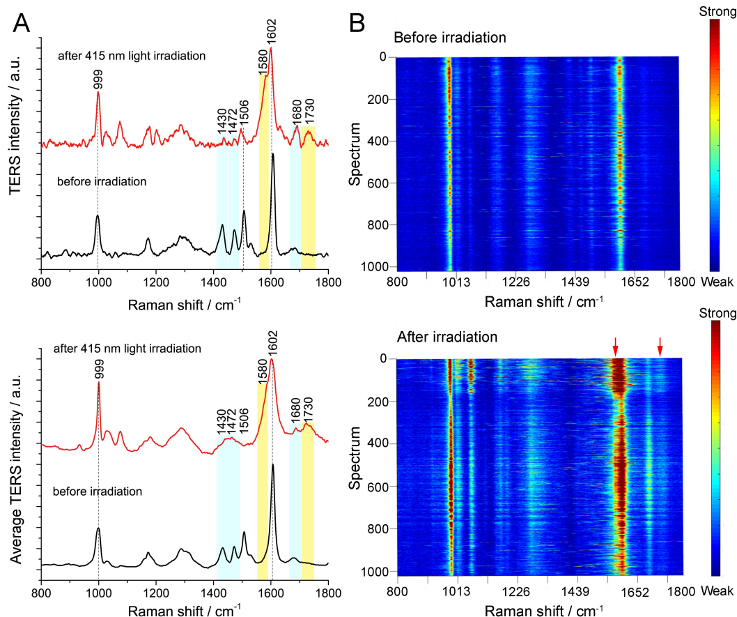
Figure 3. (A) Baseline corrected TERS spectra (top panel) of a C6 HAT monolayer on Au surface before (black) and after (red) 415 nm light irradiation, and average TERS spectra (bottom panel) from the TERS maps of a C6 HAT monolayer on Au before (black) and after (red) 415 nm light irradiation. (B) Waterfall plot of all TERS spectra from maps of a C6 HAT monolayer on Au before (top panel) and after (bottom panel) 415 nm light irradiation. The size of all maps is 1 \times 1 \mu\text{m}^2 with a 31 nm pixel size. All TERS spectra were normalized using the Raman peak at 1602 \text{ cm}^{-1} .
