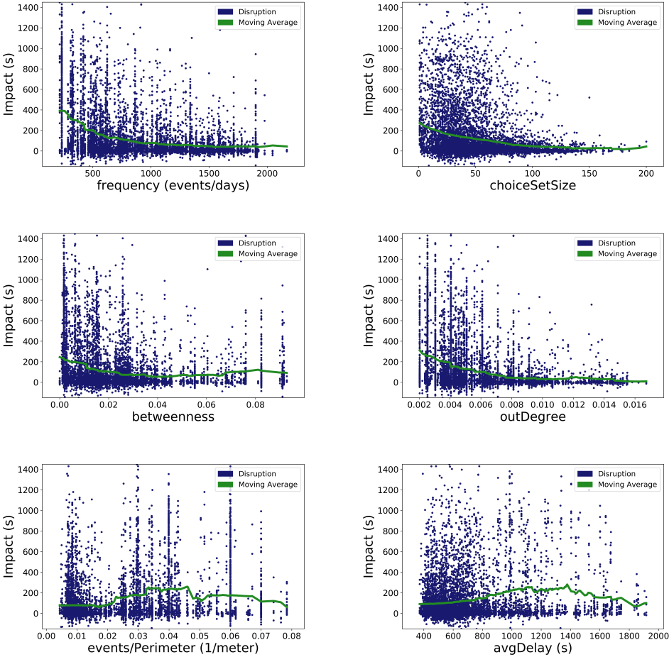
Figure 2: Relationship between features and impact.
