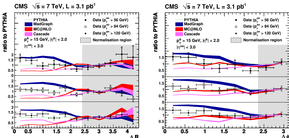
Figure 8. Ratio of the differential \overline{B\overline{B}} production cross sections, as a function of \Delta R (left) and \Delta\phi (right), for data, MADGRAPH, MC@NLO and CASCADE, with respect to the PYTHIA predictions, for the three leading jet p_T bins. The simulation is normalised to the region \Delta R > 2.4 and \Delta\phi > \frac{3}{4}\pi (FCR region), as indicated by the shaded normalisation region. The widths of the theory bands indicate the statistical uncertainties of the simulation.
