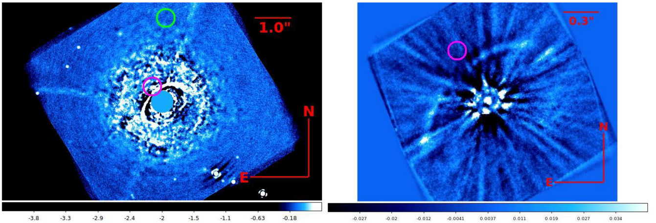
Figure 1. Final images obtained from the 2018-05-06 observations. In both cases, the values are expressed in counts. Left: IRDIS final image obtained applying the PCA algorithm and subtracting 1 mode from the original data. The green circle is to enlight the zone around the planet proposed by Pinte et al. (2018), the magenta circle enlight the zone of the planet proposed by Guidi et al. (2018). The mask covering the star has a radius of 0.37 arcsec. Right: IFS final image obtained using the PCA algorithm subtracting 1 mode from the original data. As for the IRDIS image, the magenta circle identify the zone around the planet proposed by Guidi et al. (2018).
