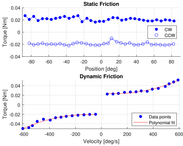
Fig. 3. Top : static friction torque as a function of the end-effector position. Bottom : dynamic friction torque as a function of the end-effector velocity.
