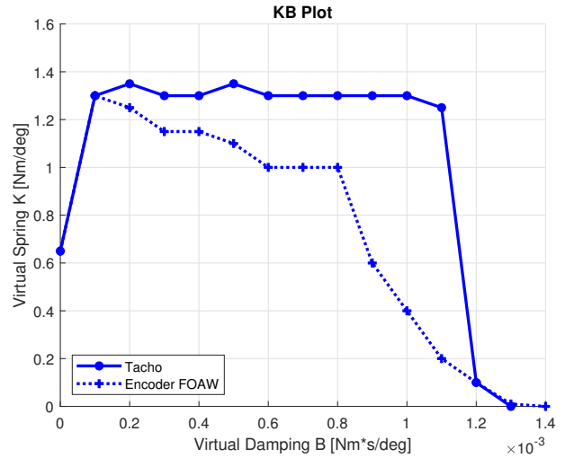
Fig. 5. KB plot visualizes the stability of a rendered virtual wall [31]. Here, impedance control with 1st order low-pass filtered tachometer signal renders the largest K-B virtual wall area.
