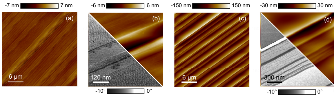
FIG. 2. (a) AFM images of an unprocessed (0001) 4H -C epitaxial surface showing a random distribution of isolated macrosteps. (b) Isolated macrostep consisting of a double-peak with atomically flat terraces and a faceted riser in between. The phase image (bottom left) also shows the microstepping of the surface away from the macrostep. (c) Surface morphology after the Si-melt process and subsequent Si removal. (d) A zoom-in view of a macrostep in (c) showing two wide terraces separated by a riser facet composed of several smaller steps. The white stripe in the phase map is a measurement artifact. Note that the scan sizes of (b) and (d) are different.
