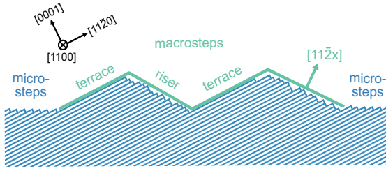
FIG. 1. Schematic of an off-axis surface showing both micro- and macrosteps as observed on commercial 4H-C epitaxial surfaces. The subnanofacets at the riser exhibit different orientations commonly described with a Miller index of (11\bar{2}x) . The terrace along the (0001) basal plane is atomically flat with only some sparsely distributed single steps as indicated on the terrace on the right. Note that the off-axis angle (the most common of these are 4^\circ ) is exaggerated in this sketch.
