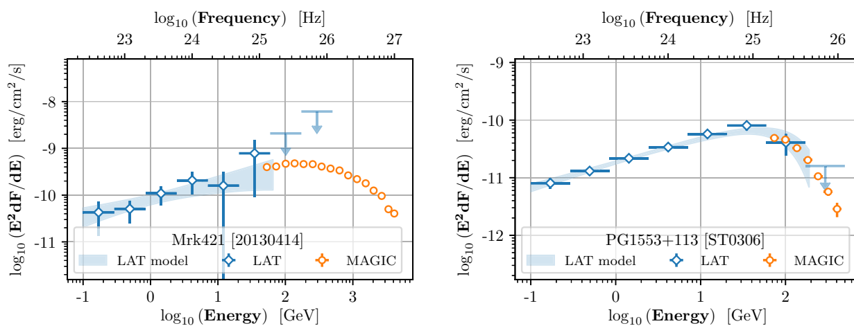
Figure 2. Detailed broad-band gamma-ray spectral energy distributions of the Markarian 421 data set of 2013 April 14 (short exposure) and the ST0306 2015 data from PG 1553+113 (long integration time), showing the good level of agreement achieved for both the MAGIC spectral points (orange open points) and the HE bow-ties and spectral points obtained through the maximum likelihood analysis of Fermi -LAT data (blue). The y-axes correspond to observed fluxes , i.e. they include the effect of absorption by the EBL. LAT upper limits are for 2\sigma confidence level.
