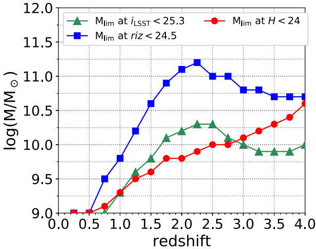
Figure 9. Redshift evolution of the stellar mass limits defined as the 90 per cent completeness threshold for galaxy samples selected in Euclid H (red line and circles), r_{\text{iz}} (blue line and squares), and LSST i filter (green line and triangles).
