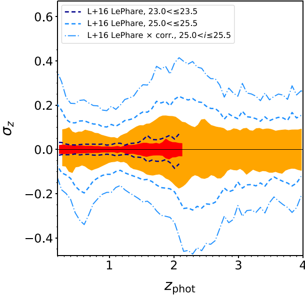
Figure 4. Median photometric redshift 1\sigma uncertainty of HORIZON-AGN galaxies at 23 < i^+ \leq 23.5 and 25 < i^+ \leq 25.5 , as a function of z_{\text{phot}} (shaded areas, colours as in Fig. 3). Dashed lines show the median \sigma_{z, \text{L16}} of real COSMOS2015 galaxies in the same magnitude bins (dark blue: 23 < i^+ \leq 23.5 , and light blue: 25 < i^+ \leq 25.5 ). Both HORIZON-AGN and COSMOS2015 errors are computed by LEPHARE using the z_{\text{phot}} likelihood function. The dotted–dashed lines embrace the median of COSMOS2015 enhanced errors at 25 < i^+ \leq 25.5 , i.e. the original \sigma_{z, \text{L16}} values have been increased by a multiplicative ‘boosting factor’ as prescribed in L16. See Section 3.1.2 for more details. Note that the y-axis range is different from Fig. 3.
