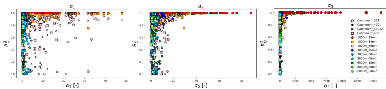
Fig 2: Scaling factors in relation with the coefficient of determination R^2
