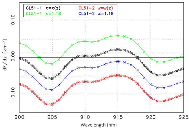
Figure 12. First derivative, dF(z, \lambda_{\text{on}})/dz (see Eq. 15), of the ratio of the CL51 ceilometer signal and the extrapolated reference lidar signal as a function of \lambda_{\text{on}} : CL51-1 (solid black line) and CL51-2 (solid red line) assuming a height-dependent \kappa(z) . The short-dashed and long-dashed lines are for the minimum and maximum S_p values, respectively. The integer wavelength corresponding to the minimum of the absolute values of dF/dz is indicated by a circle. The green (CL51-1) and blue (CL51-2) lines correspond to dF/dz assuming a constant \kappa derived from AERONET. All curves concern Case A.
