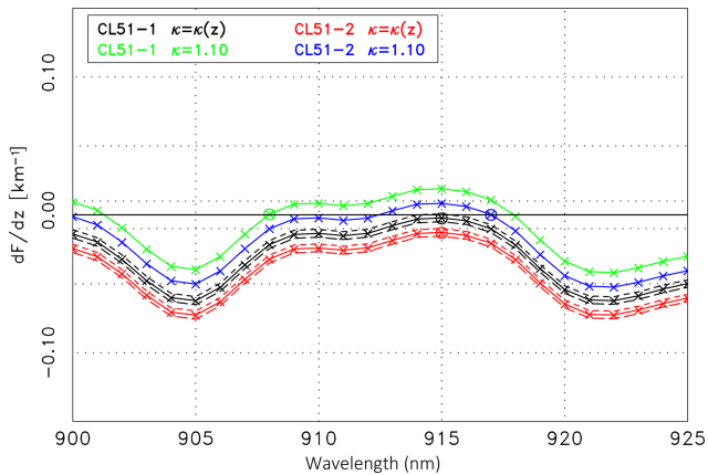
Figure 16. First derivative dF(z, \lambda_{on})/dz (see Eq. 15), of the ratio of the CL51 ceilometer signal and the extrapolated reference lidar signal as a function of \lambda_{on} : analogously to Fig. 12, but for 20 August 2015, 05:00–08:00 UTC (Case B). The corresponding CL51 ceilometers and Angström exponent settings are indicated in the legend.
