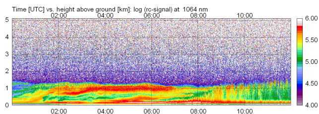
Figure 9. Time–height cross section of the range-corrected signal (in arbitrary units, logarithmic scale) of CHX-1 from 2 July 2015 (including Case A) to noon. Time is given in UTC, and the height above ground in kilometers; note that the vertical range shown here is not the full measurement range of the ceilometer.
