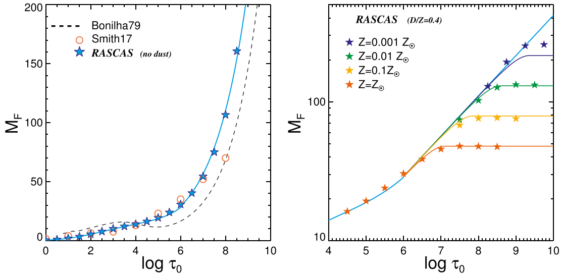
Figure 1. Multiplication factor ( M_F ) of Ly \alpha photons as a function of optical depth at the line centre ( \tau_0 ), computed using the Monte Carlo Ly \alpha radiative transfer code, RASCAS. Left: M_F in the dust-free medium with temperature T = 100 K. The dashed line indicates the results ( t_{\text{trap}}/t_{\text{light}} \approx M_F ) from an earlier work by Bonilha et al. (1979) with temperature T = 10^4 K, and the empty circles correspond to the results ( t_{\text{trap}}/t_{\text{light}} ) at T = 1 K from Smith et al. (2017b). The solid line indicates the fit to our calculations (equations 6 and 7). Right: M_F in the presence of dust. The star symbols with different colour codings are the results from our Monte Carlo calculations with different metallicities assuming a constant dust-to-metal ratio of 0.4. The solid lines are the fits to these results (see the text). Note that each Ly \alpha photon can transfer \sim 10 –300 times larger momentum than the single scattering case in metal-poor environments.
