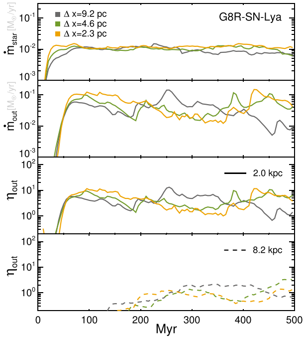
Figure A1. Resolution test of the runs with Ly \alpha pressure. From top to bottom, each panel shows the SF rates in M_{\odot} \text{ yr}^{-1} , the outflow rates measured at |z| = 2 \text{ kpc} , the mass-loading factors measured at |z| = 2 \text{ kpc} and |z| = 0.2 R_{\text{vir}} (8.2 kpc).
