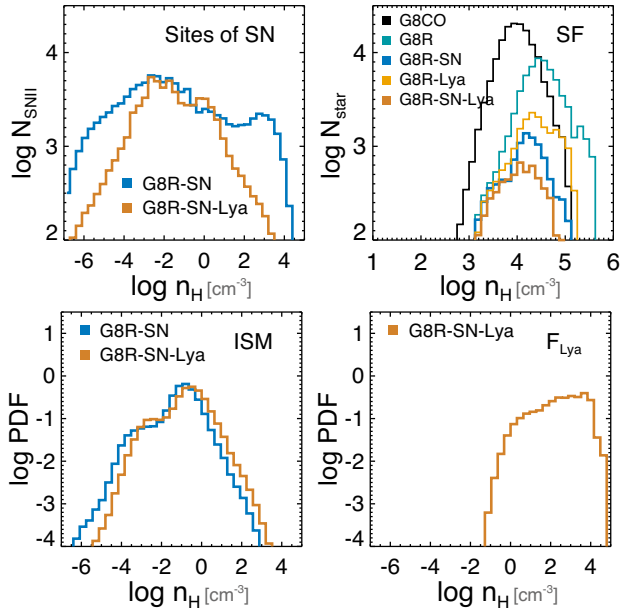
Figure 6. Distributions of densities at which SN explodes (top left) and star particles are formed (top right). The dense gas ( n_{\text{H}} \gtrsim 100 \text{ cm}^{-3} ) is efficiently dispersed before the onset of SNe in the presence of Ly \alpha pressure in the metal-poor system. The fraction of star particles formed at very high densities ( n_{\text{H}} \gtrsim 10^4 \text{ cm}^{-3} ) is also reduced. The bottom left panel shows the volume-weighted density distributions of the ISM around the central mid-plane ( \sqrt{x^2 + y^2} < r_{\text{half, m}} and |z| < H ), where r_{\text{half, m}} is the half-mass radius and H is the scale height (see the text). The bottom right panel indicates the volume-weighted densities at which Ly \alpha force ( \propto N_{\text{Ly}\alpha} M_{\text{F}} ) is significant.
