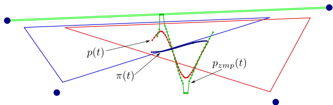
Fig. 3. The solution obtained by the motion planner when a dynamic lateral walk gait is active. The support polygons are computed as the convex hull of the points which are in contact (large blue dots) according to the contact schedule. To increase robustness of the solution, a safety margin is applied to the polygons such that their area is reduced. Only the first three support polygons of the sequence (respectively in red, green and blue) are shown. The resulting center of mass motion \mathbf{p}(t) (red path) is optimized to deviate the least possible from a path regularizer \pi(t) (blue path), while the ZMP \mathbf{p}_{zmp}(t) (green path) is constrained to always lie in the active support polygon. When two lateral legs are simultaneously swinging, the support polygon collapses to a line (shown in green). To avoid numerical issues and excessive accelerations due to a required increase in the order of the approximating spline, we expand the line to a rectangle.
