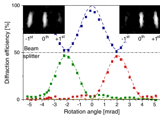
FIG. 2 (color online). Angular dependence of the 0th and \pm 1 st order diffraction efficiencies for cold neutrons at \lambda = 2 \text{ nm} for gratings assembled from a SiO 2 nanoparticle-polymer composite with a spacing of \Lambda = 500 \text{ nm} and an effective thickness of d = 203 \mu\text{m} (S7). Lines are a simultaneous RCWA fit to the data. Inset: Detector matrix (gray scale of logarithmic box counts at Bragg positions).
