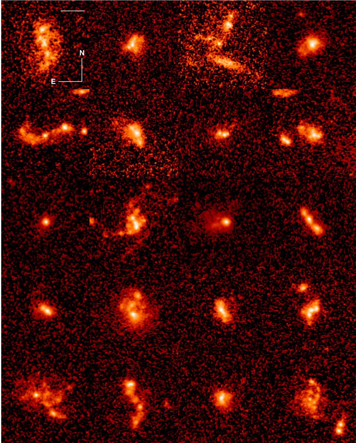
Figure A1. HST / i 814 cutouts of bright H \alpha emitters in COSMOS. The cutouts show a random sample of emitters with predicted H \alpha fluxes \geq 2 \times 10^{-16} erg cm ^{-2} s ^{-1} at 1.4 < z < 1.8 . The size is 3.75 arcsec \times 3.75 arcsec. The images are aligned North-East and they are scaled to the same background level. The white bar shown in the top left-hand panel is 1 arcsec long.
