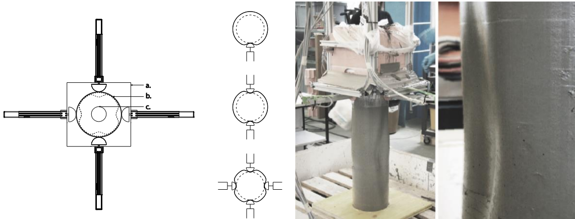
Figure 2: Left: Schematic view of the flexible formwork; four actuators were mounted in equal distance around the formwork, with three diagrams showing the possible configurations. Right: production with flexible formwork [10]
