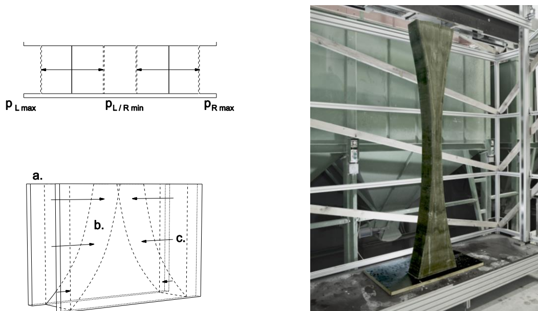
Figure 4: Upper left, schematic top view of flexible formwork. P_{L/R \max} , is the maximum volume increase, while P_{L/R \min} , indicates the minimum volume decrease. P_L and P_R are controlled individually, thus the design space is not constrained to a symmetric structure. Lower left: a schematic illustration of the formwork; a) rigid box; b) flexible metal; c) arrows indicate position of actuators manipulating the flexible metal globally over the height of the formwork. Right: a 2-meter tall structure produced with the flexible formwork [13].
