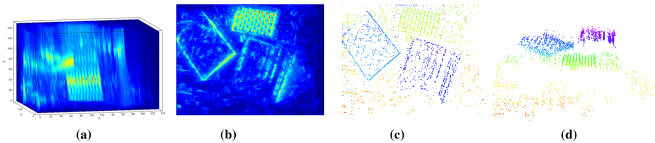
Fig. 6 Our method builds the ray density DSI (a), from which a confidence map (b) and a semi-dense depth map (c) are extracted in a virtual camera. The semi-dense depth map gives a point cloud of scene edges
