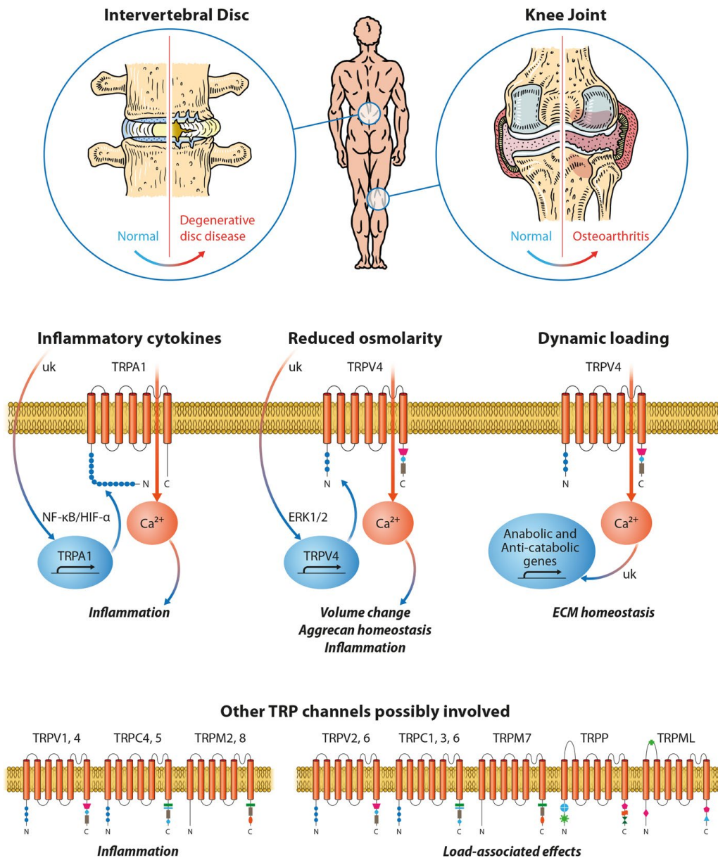
Fig. 2. Function of TRP channels in joint diseases. The gene expression of TRPA1 in cartilaginous tissues can be stimulated by inflammatory cytokines and regulated by NF- \kappa B and HIF- \alpha . Active TRPA1 further promote inflammatory responses. The expression of TRPV4 is influenced by osmolarity and regulated by ERK1/2. Active TRPV4 is implicated in cellular volume change, aggrecan homeostasis and inflammatory responses. Ca^{2+} influx through TRPV4 can be directly stimulated by physiological loading, promoting expression of anabolic and anti-catabolic genes. Evidence suggests that other TRP channels also contribute to inflammation and load-induced effects in degenerative disc disease and osteoarthritis, but their involvement is not completely understood. uk = exact mechanism unknown.
