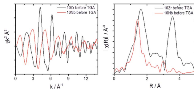
Fig. 9 EXAFS comparison of 10Zr and 10Nb in k space and for Fourier transformed data.
