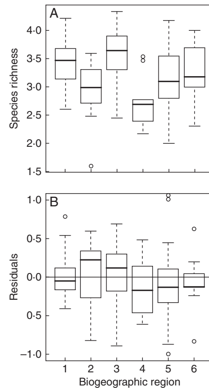
FIG. 2. Box-and-whisker plots in the different biogeographical regions (1, Nearctic; 2, Neotropical; 3, Palearctic; 4, Ethiopian; 5, Oriental; 6, Australasian) of (A) botanic garden species richness ( n = 179 ) and (B) residuals of the models presented in Table 1 for the same gardens.
